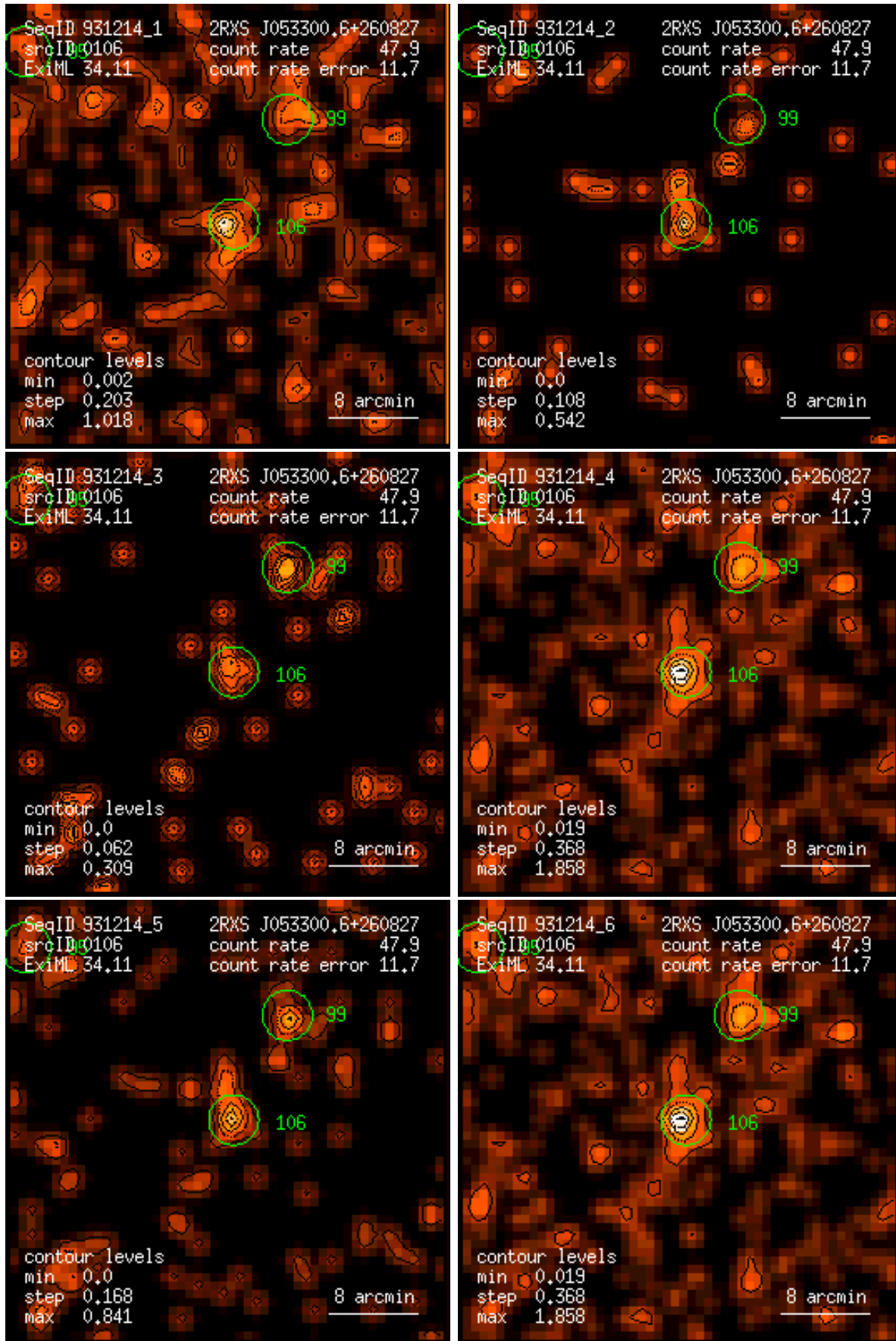
Figure 106: RASS 931214: detection 0106: band rate images, Gaussian filter: (1) PSPC channels 11 – 41, (2) 52 – 90, (3) 91 – 201, (4) 11 – 235, (5) 52 – 201, (6) 11 – 201. Broad band rates in counts/ks. Band rate contour levels in counts/ks/arcmin 2 .
