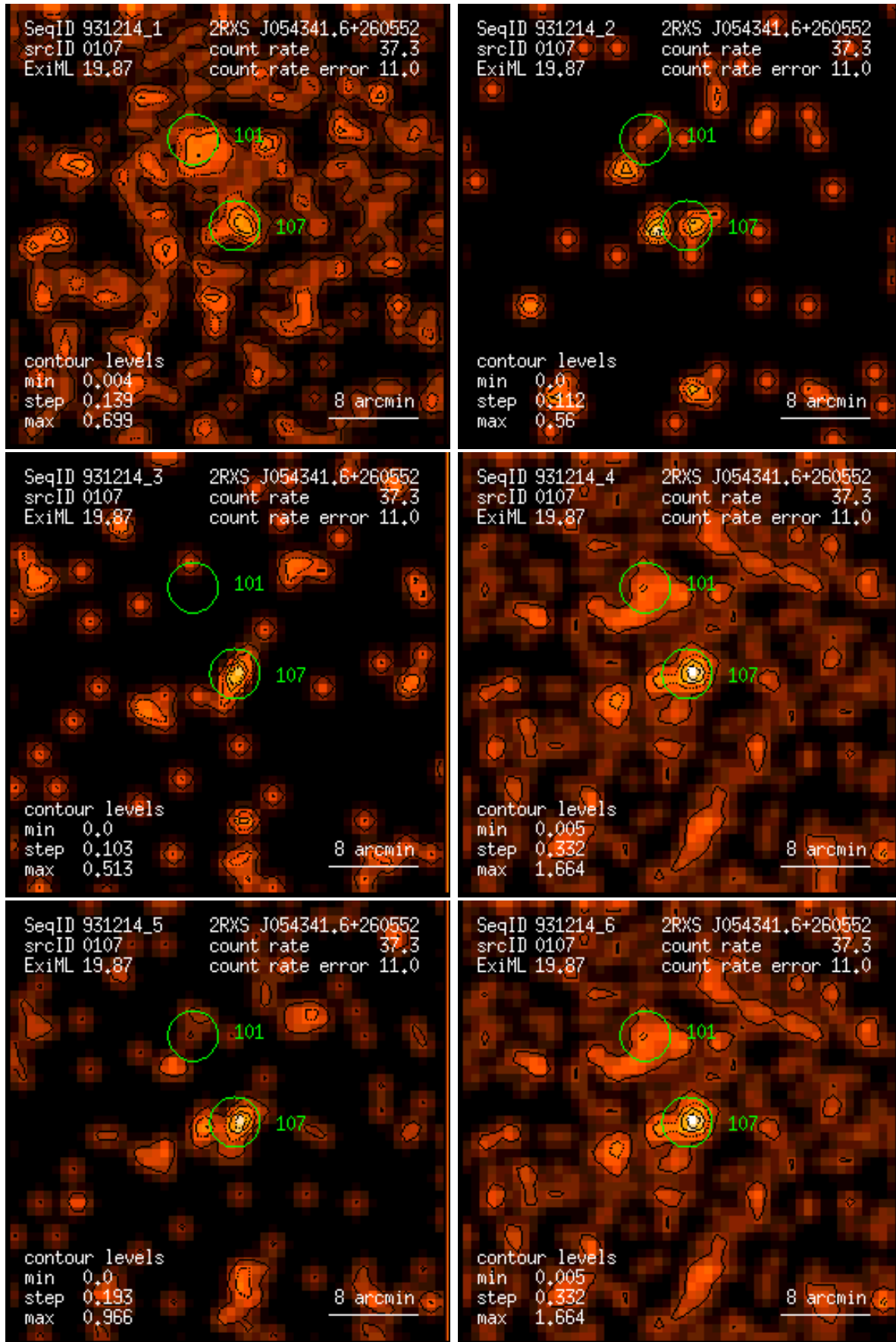
Figure 107: RASS 931214: detection 0107: band rate images, Gaussian filter: (1) PSPC channels 11 – 41, (2) 52 – 90, (3) 91 – 201, (4) 11 – 235, (5) 52 – 201, (6) 11 – 201. Broad band rates in counts/ks. Band rate contour levels in counts/ks/arcmin 2 .
