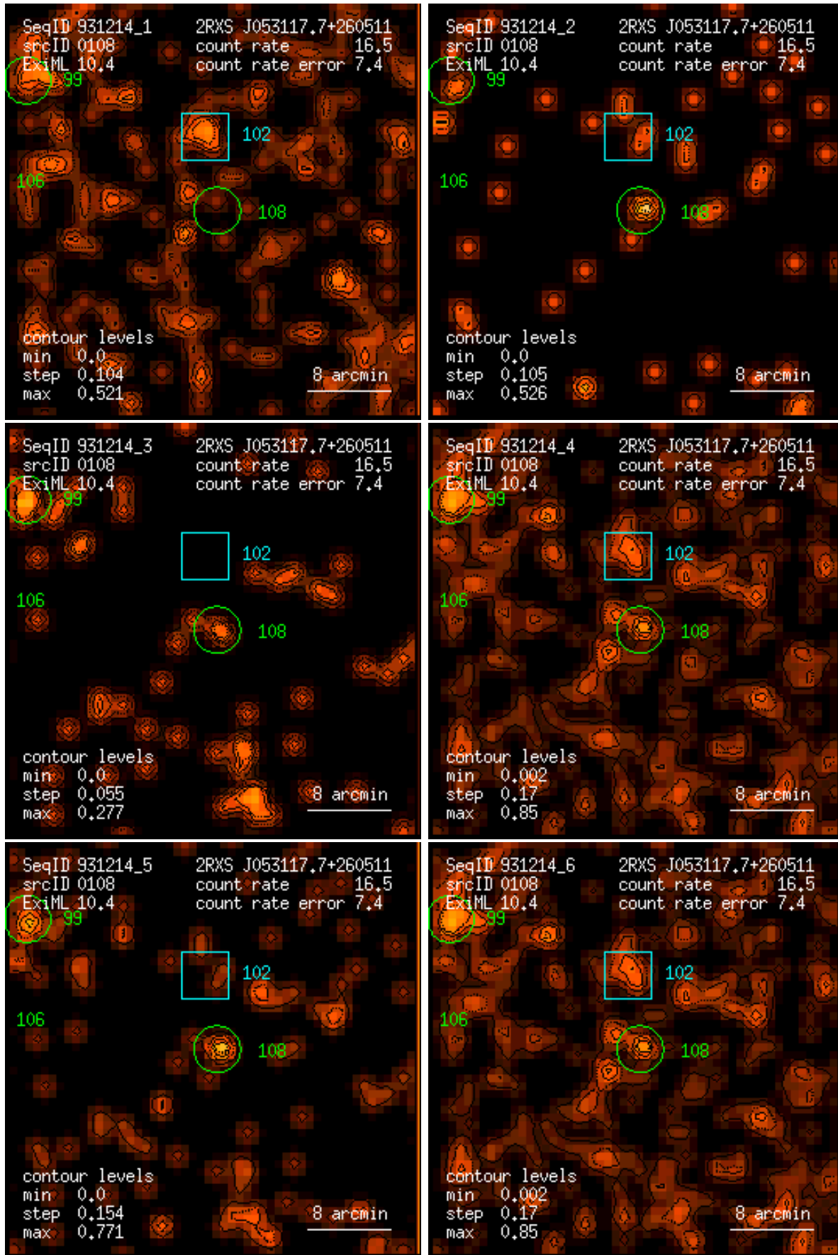
Figure 108: RASS 931214: detection 0108: band rate images, Gaussian filter: (1) PSPC channels 11 – 41, (2) 52 – 90, (3) 91 – 201, (4) 11 – 235, (5) 52 – 201, (6) 11 – 201. Broad band rates in counts/ks. Band rate contour levels in counts/ks/arcmin 2 .
