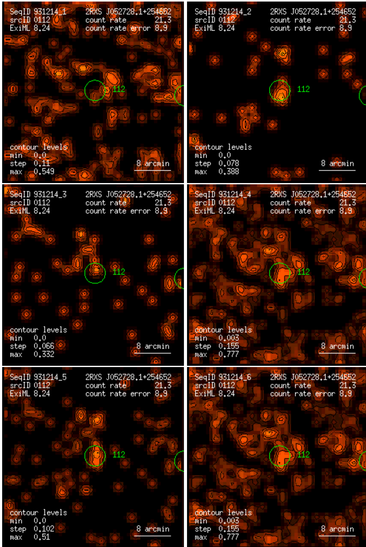
Figure 112: RASS 931214: detection 0112: band rate images, Gaussian filter: (1) PSPC channels 11 – 41, (2) 52 – 90, (3) 91 – 201, (4) 11 – 235, (5) 52 – 201, (6) 11 – 201. Broad band rates in counts/ks. Band rate contour levels in counts/ks/arcmin 2 .
