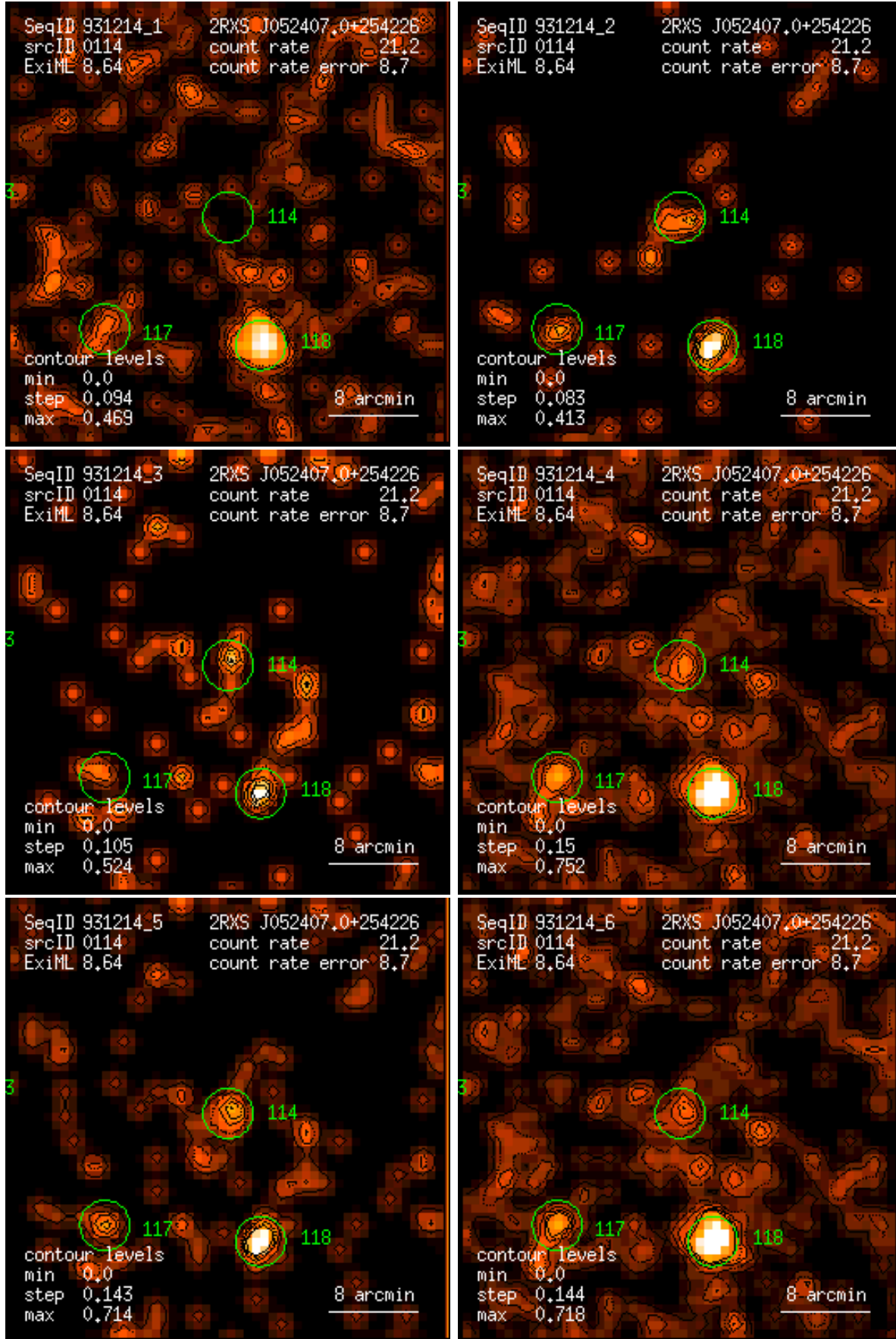
Figure 114: RASS 931214: detection 0114: band rate images, Gaussian filter: (1) PSPC channels 11 – 41, (2) 52 – 90, (3) 91 – 201, (4) 11 – 235, (5) 52 – 201, (6) 11 – 201. Broad band rates in counts/ks. Band rate contour levels in counts/ks/arcmin 2 .
