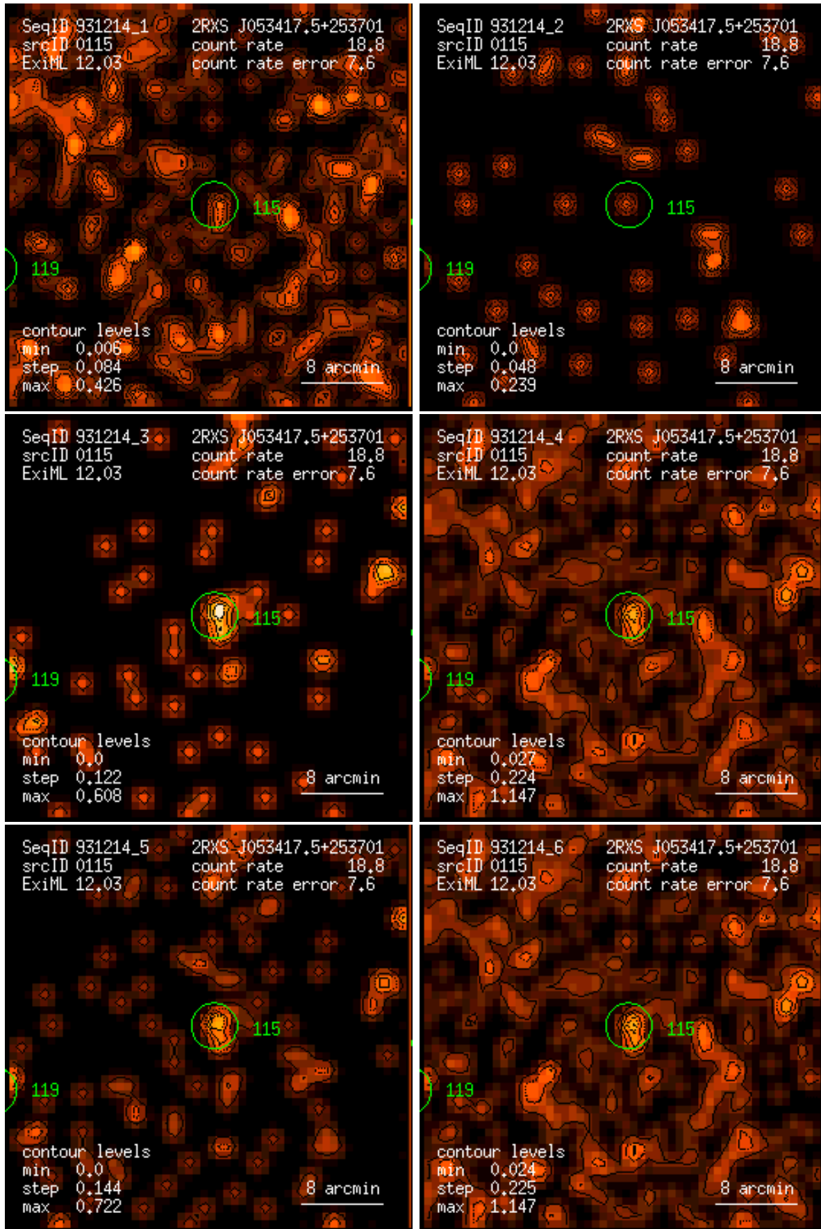
Figure 115: RASS 931214: detection 0115: band rate images, Gaussian filter: (1) PSPC channels 11 – 41, (2) 52 – 90, (3) 91 – 201, (4) 11 – 235, (5) 52 – 201, (6) 11 – 201. Broad band rates in counts/ks. Band rate contour levels in counts/ks/arcmin 2 .
