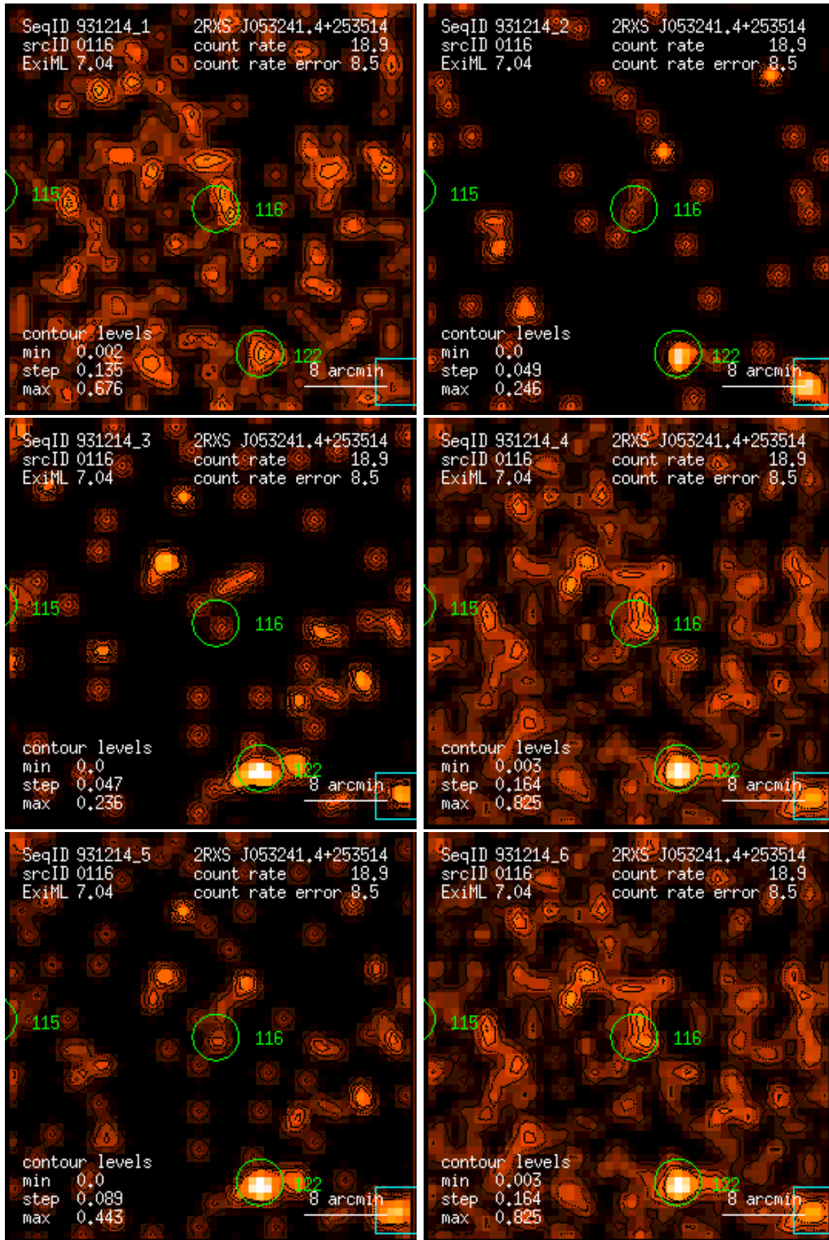
Figure 116: RASS 931214: detection 0116: band rate images, Gaussian filter: (1) PSPC channels 11 – 41, (2) 52 – 90, (3) 91 – 201, (4) 11 – 235, (5) 52 – 201, (6) 11 – 201. Broad band rates in counts/ks. Band rate contour levels in counts/ks/arcmin 2 .
