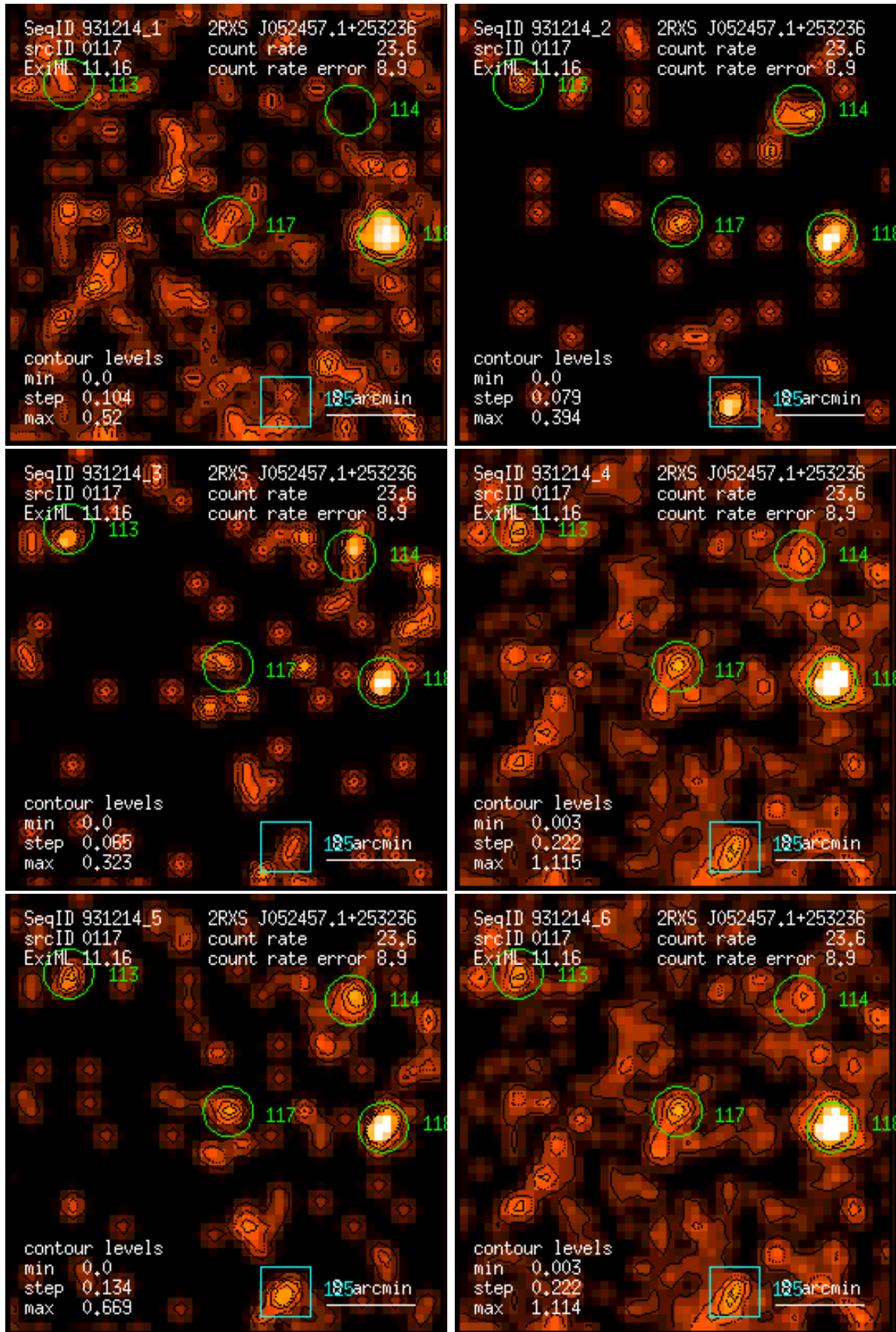
Figure 117: RASS 931214: detection 0117: band rate images, Gaussian filter: (1) PSPC channels 11 – 41, (2) 52 – 90, (3) 91 – 201, (4) 11 – 235, (5) 52 – 201, (6) 11 – 201. Broad band rates in counts/ks. Band rate contour levels in counts/ks/arcmin 2 .
