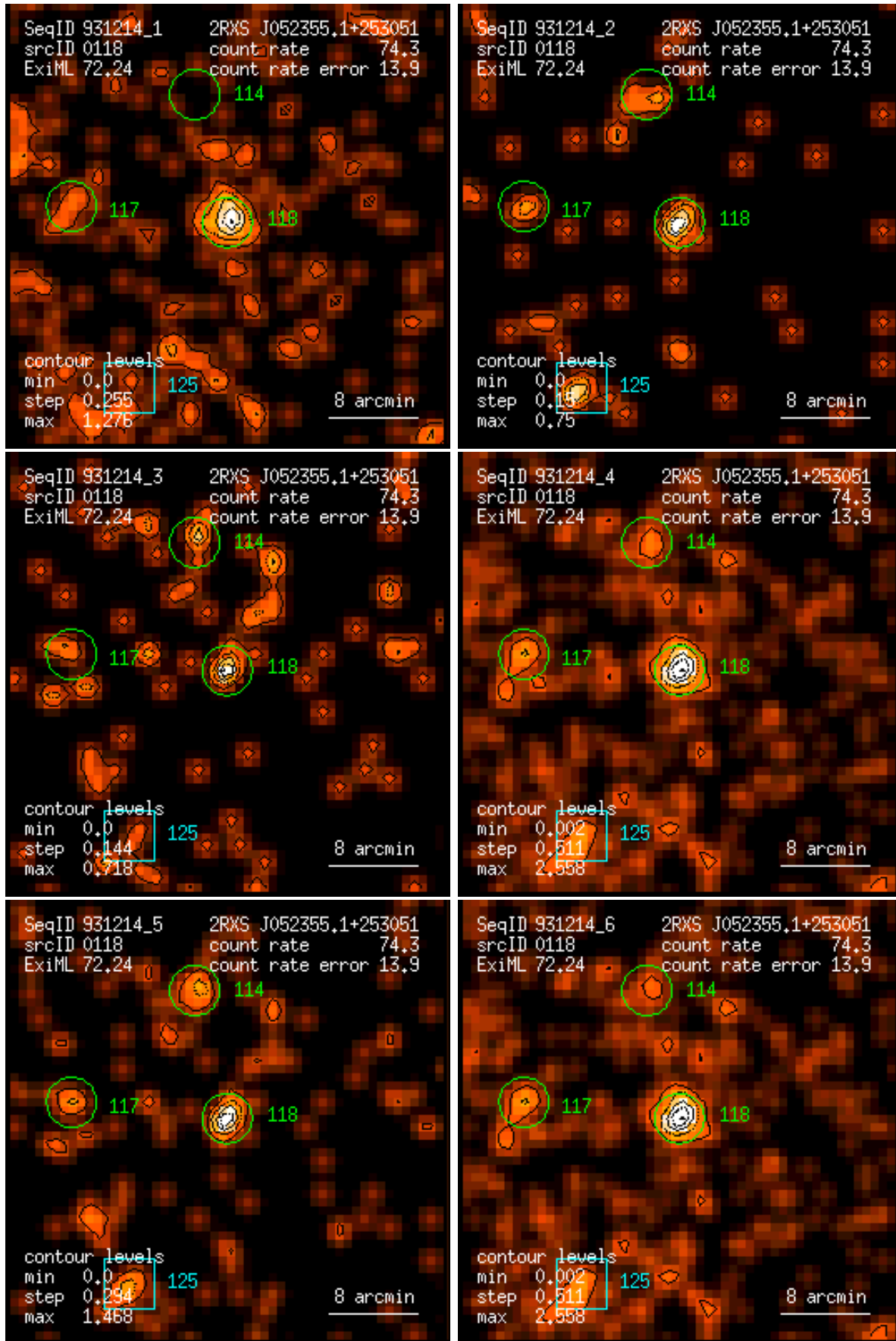
Figure 118: RASS 931214: detection 0118: band rate images, Gaussian filter: (1) PSPC channels 11 – 41, (2) 52 – 90, (3) 91 – 201, (4) 11 – 235, (5) 52 – 201, (6) 11 – 201. Broad band rates in counts/ks. Band rate contour levels in counts/ks/arcmin 2 .
