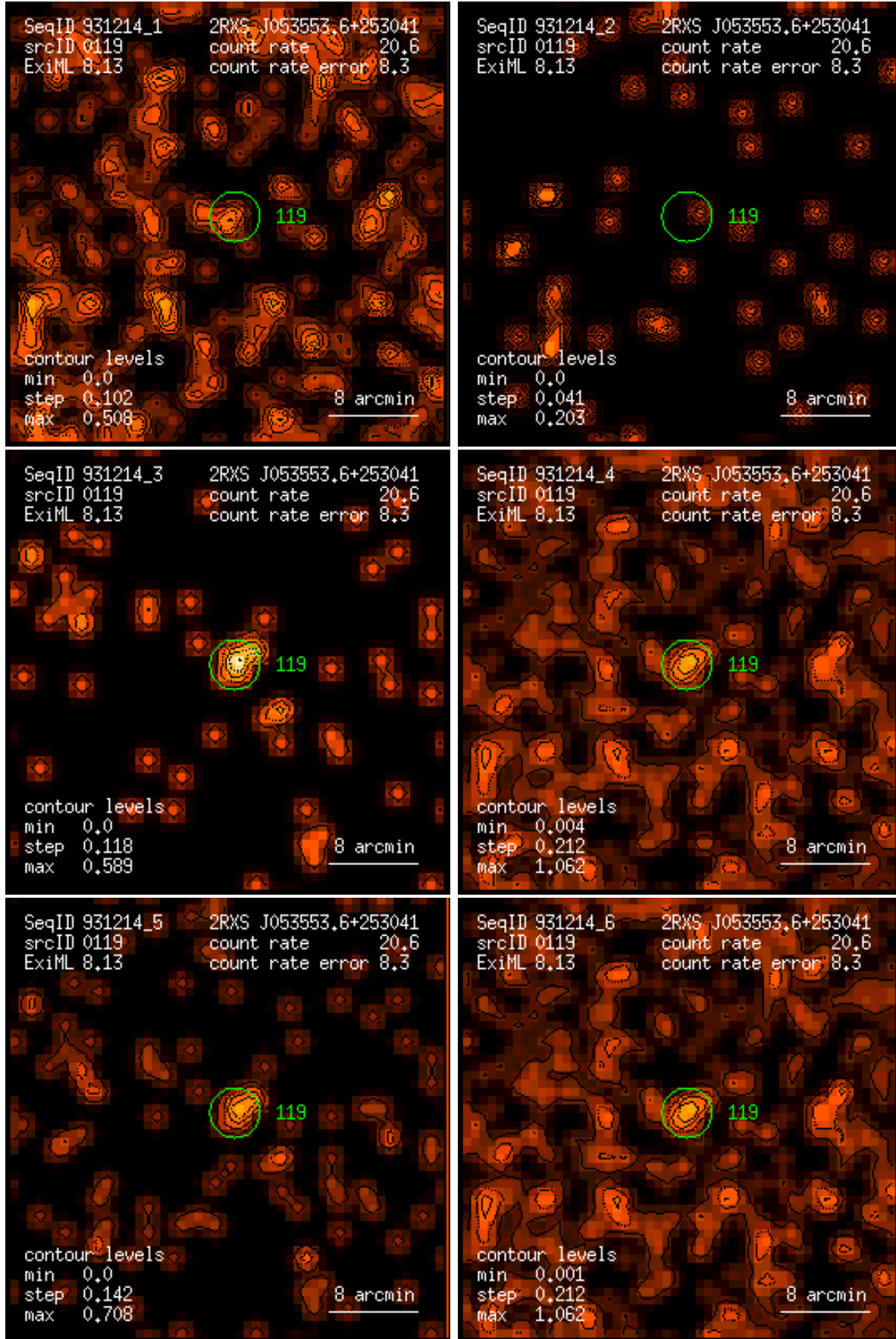
Figure 119: RASS 931214: detection 0119: band rate images, Gaussian filter: (1) PSPC channels 11 – 41, (2) 52 – 90, (3) 91 – 201, (4) 11 – 235, (5) 52 – 201, (6) 11 – 201. Broad band rates in counts/ks. Band rate contour levels in counts/ks/arcmin 2 .
