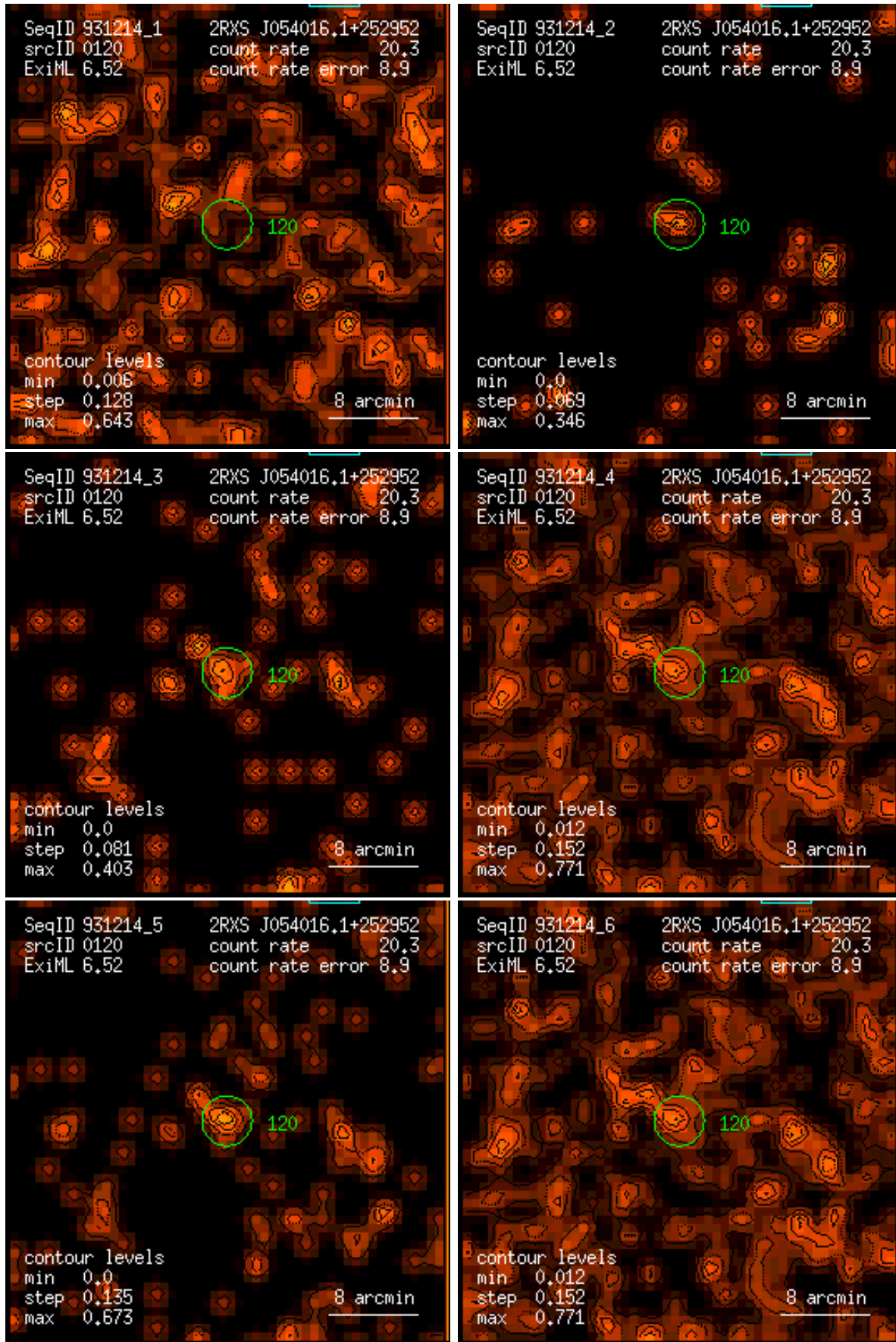
Figure 120: RASS 931214: detection 0120: band rate images, Gaussian filter: (1) PSPC channels 11 – 41, (2) 52 – 90, (3) 91 – 201, (4) 11 – 235, (5) 52 – 201, (6) 11 – 201. Broad band rates in counts/ks. Band rate contour levels in counts/ks/arcmin 2 .
