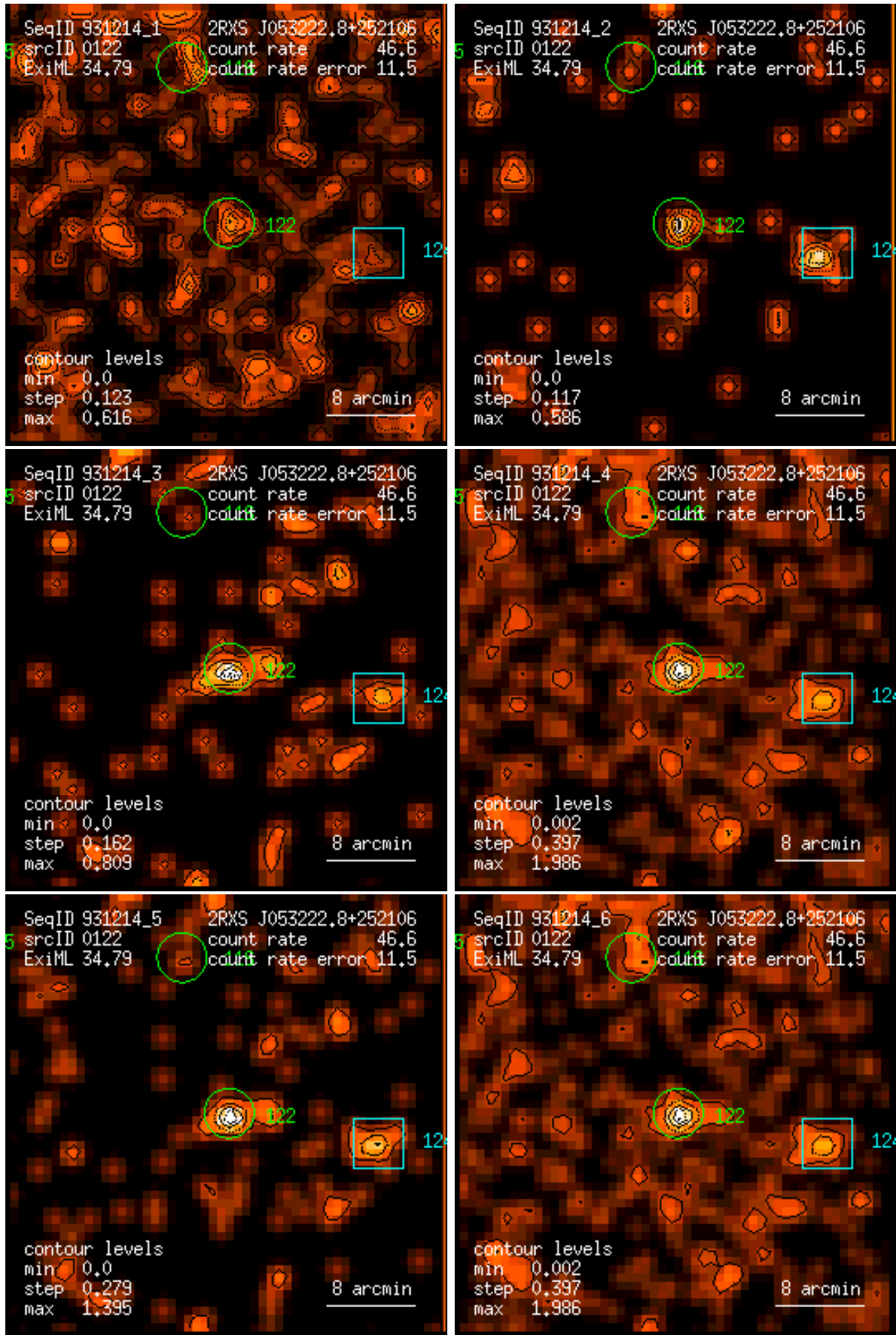
Figure 122: RASS 931214: detection 0122: band rate images, Gaussian filter: (1) PSPC channels 11 – 41, (2) 52 – 90, (3) 91 – 201, (4) 11 – 235, (5) 52 – 201, (6) 11 – 201. Broad band rates in counts/ks. Band rate contour levels in counts/ks/arcmin 2 .
