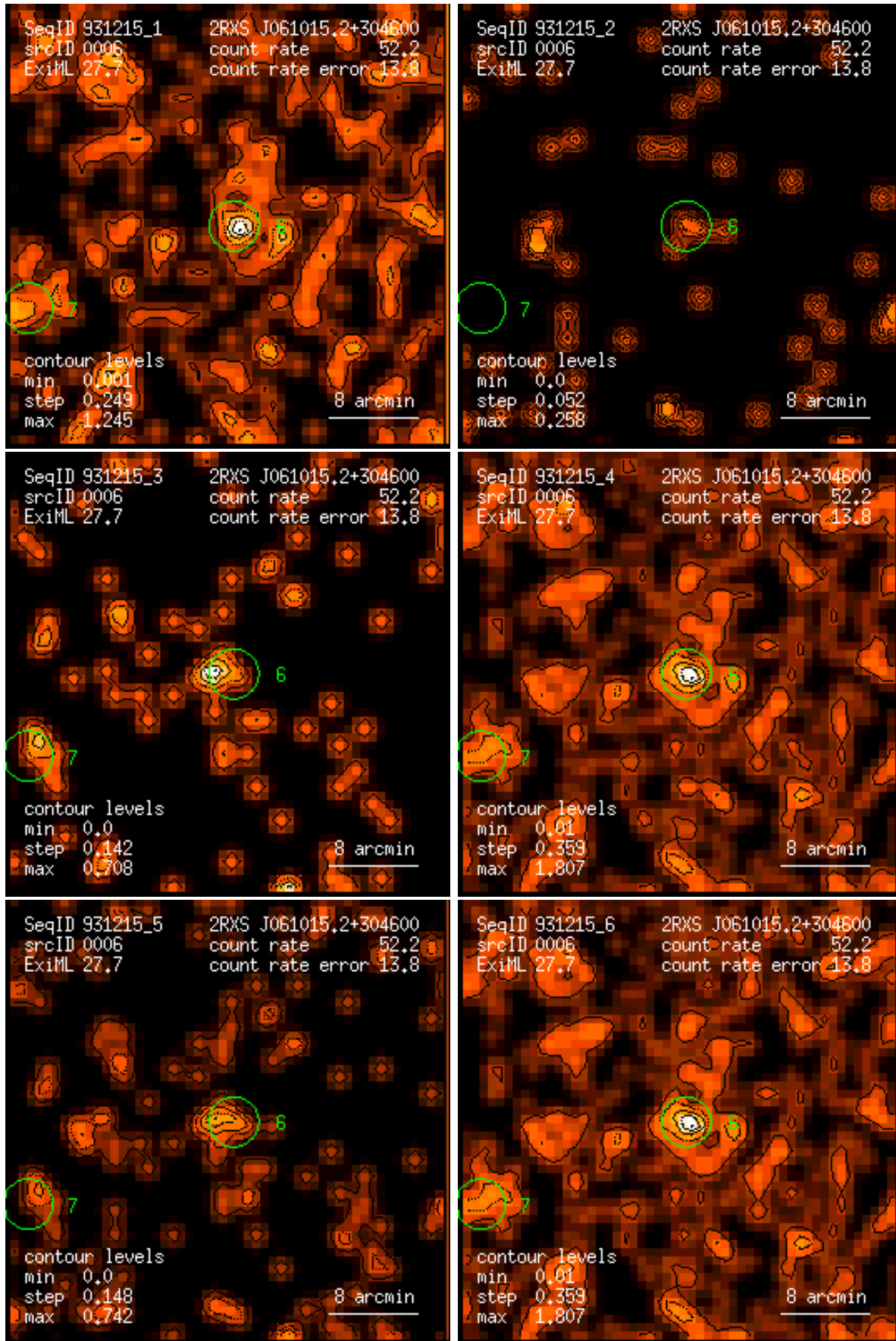
Figure 6: RASS 931215: detection 0006: band rate images, Gaussian filter: (1) PSPC channels 11 – 41, (2) 52 – 90, (3) 91 – 201, (4) 11 – 235, (5) 52 – 201, (6) 11 – 201. Broad band rates in counts/ks. Band rate contour levels in counts/ks/arcmin 2 .
