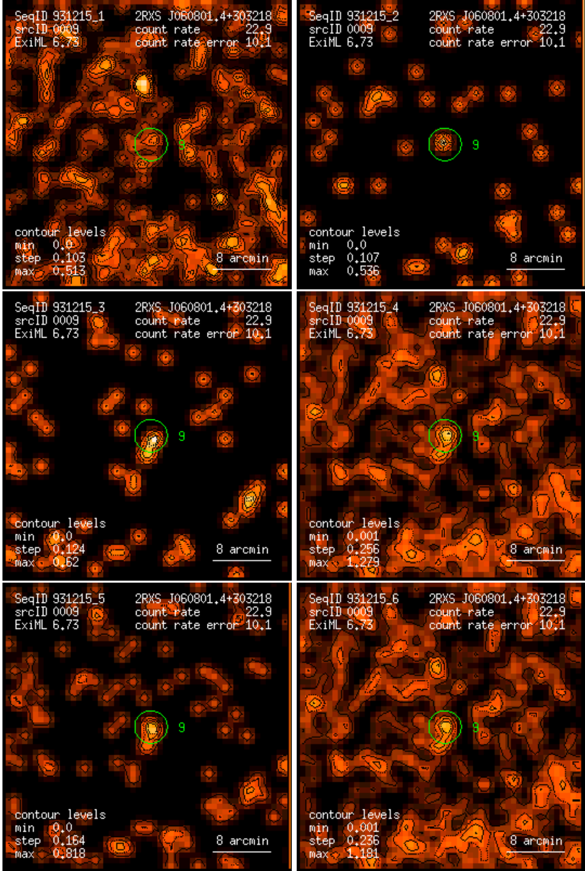
Figure 9: RASS 931215: detection 0009: band rate images, Gaussian filter: (1) PSPC channels 11 – 41, (2) 52 – 90, (3) 91 – 201, (4) 11 – 235, (5) 52 – 201, (6) 11 – 201. Broad band rates in counts/ks. Band rate contour levels in counts/ks/arcmin 2 .
