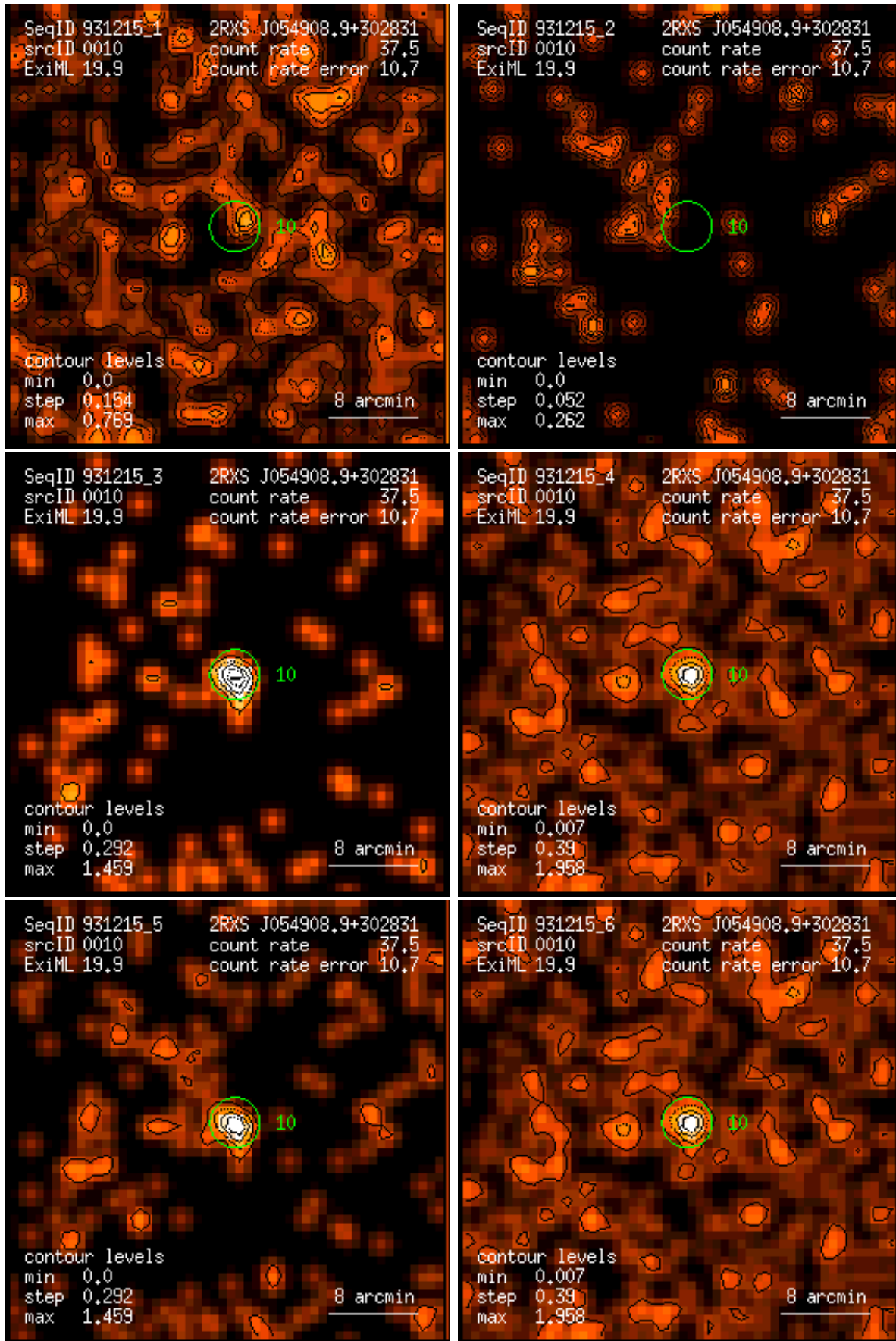
Figure 10: RASS 931215: detection 0010: band rate images, Gaussian filter: (1) PSPC channels 11 – 41, (2) 52 – 90, (3) 91 – 201, (4) 11 – 235, (5) 52 – 201, (6) 11 – 201. Broad band rates in counts/ks. Band rate contour levels in counts/ks/arcmin 2 .
