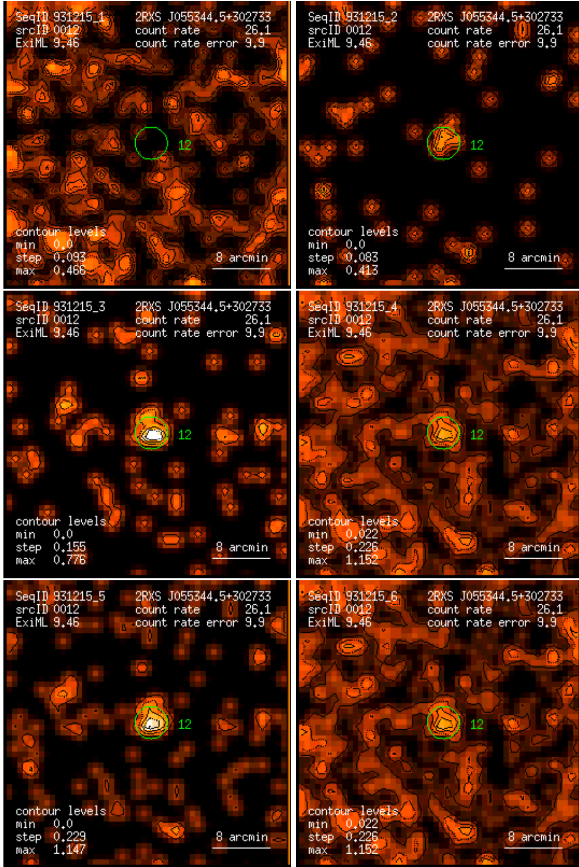
Figure 12: RASS 931215: detection 0012: band rate images, Gaussian filter: (1) PSPC channels 11 – 41, (2) 52 – 90, (3) 91 – 201, (4) 11 – 235, (5) 52 – 201, (6) 11 – 201. Broad band rates in counts/ks. Band rate contour levels in counts/ks/arcmin 2 .
