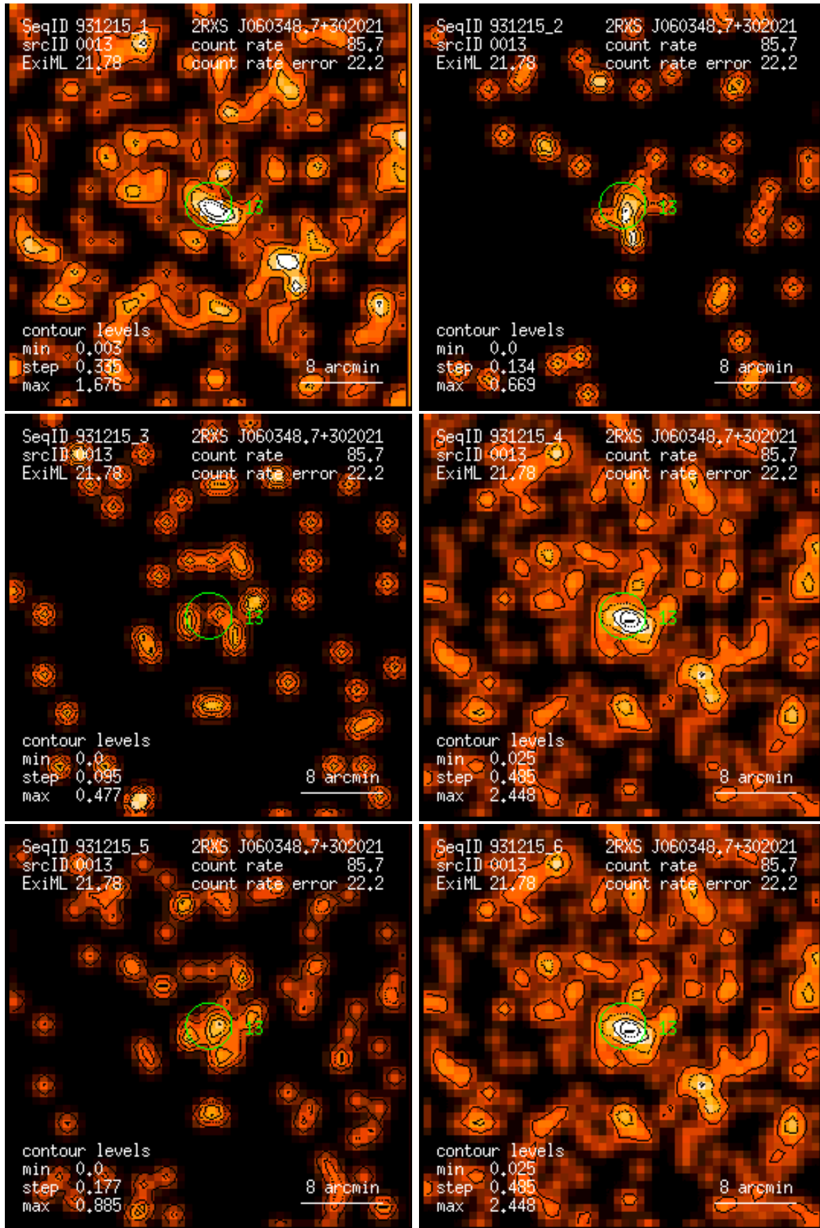
Figure 13: RASS 931215: detection 0013: band rate images, Gaussian filter: (1) PSPC channels 11 – 41, (2) 52 – 90, (3) 91 – 201, (4) 11 – 235, (5) 52 – 201, (6) 11 – 201. Broad band rates in counts/ks. Band rate contour levels in counts/ks/arcmin 2 .
