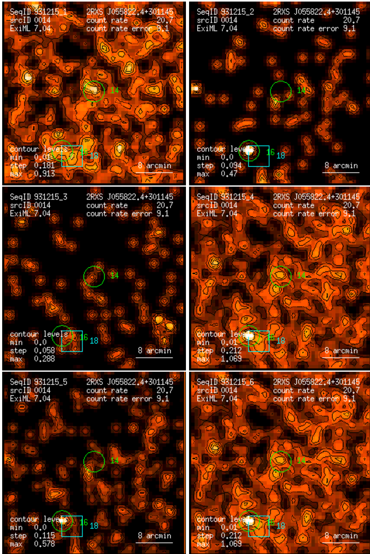
Figure 14: RASS 931215: detection 0014: band rate images, Gaussian filter: (1) PSPC channels 11 – 41, (2) 52 – 90, (3) 91 – 201, (4) 11 – 235, (5) 52 – 201, (6) 11 – 201. Broad band rates in counts/ks. Band rate contour levels in counts/ks/arcmin 2 .
