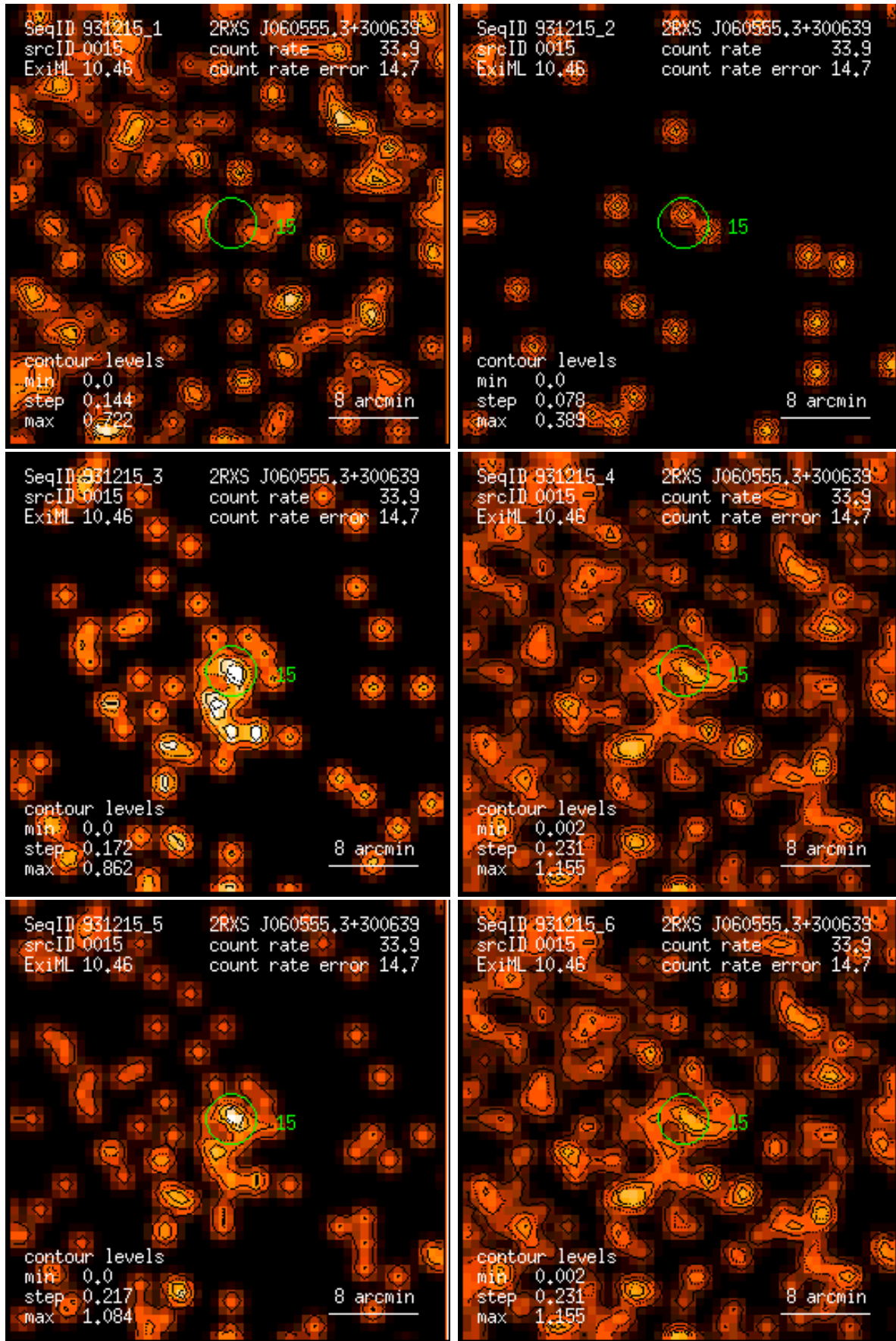
Figure 15: RASS 931215: detection 0015: band rate images, Gaussian filter: (1) PSPC channels 11 – 41, (2) 52 – 90, (3) 91 – 201, (4) 11 – 235, (5) 52 – 201, (6) 11 – 201. Broad band rates in counts/ks. Band rate contour levels in counts/ks/arcmin 2 .
