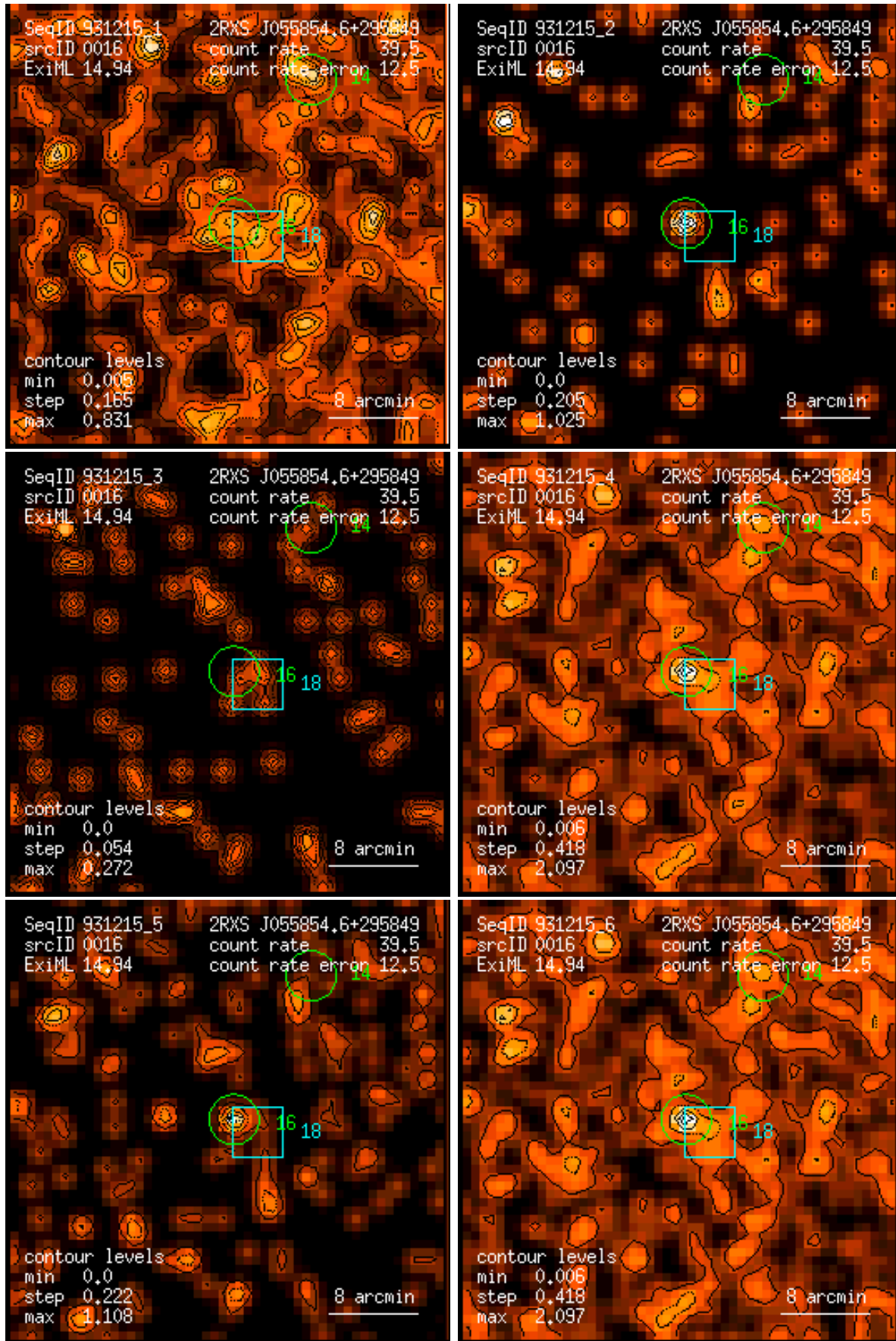
Figure 16: RASS 931215: detection 0016: band rate images, Gaussian filter: (1) PSPC channels 11 – 41, (2) 52 – 90, (3) 91 – 201, (4) 11 – 235, (5) 52 – 201, (6) 11 – 201. Broad band rates in counts/ks. Band rate contour levels in counts/ks/arcmin 2 .
