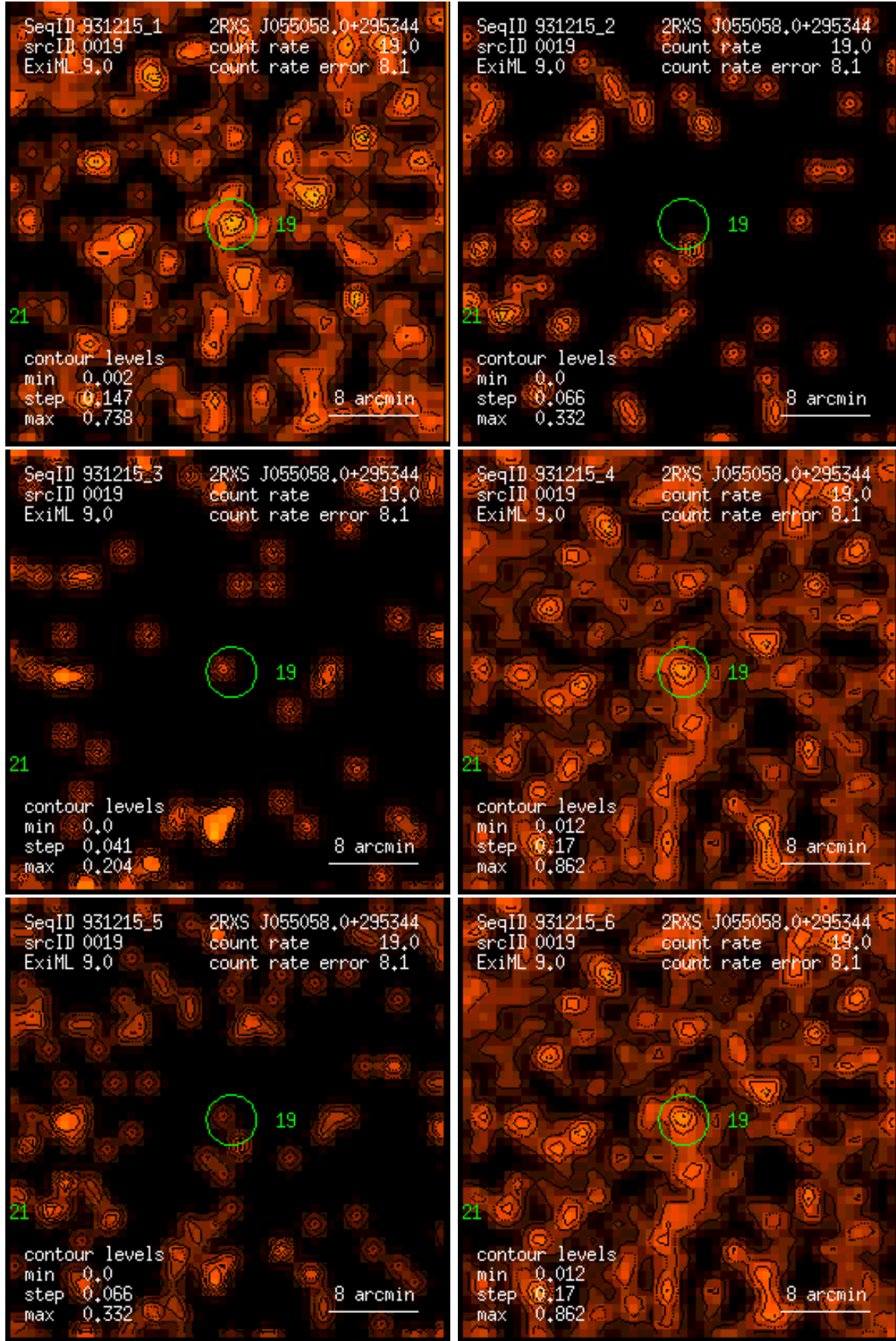
Figure 19: RASS 931215: detection 0019: band rate images, Gaussian filter: (1) PSPC channels 11 – 41, (2) 52 – 90, (3) 91 – 201, (4) 11 – 235, (5) 52 – 201, (6) 11 – 201. Broad band rates in counts/ks. Band rate contour levels in counts/ks/arcmin 2 .
