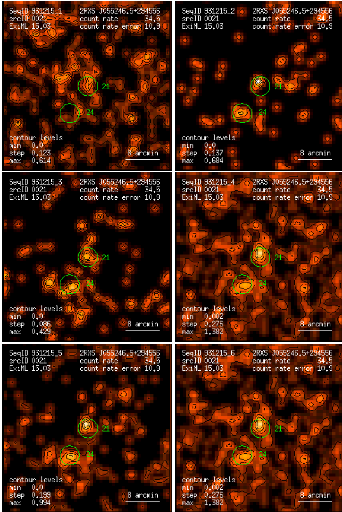
Figure 21: RASS 931215: detection 0021: band rate images, Gaussian filter: (1) PSPC channels 11 – 41, (2) 52 – 90, (3) 91 – 201, (4) 11 – 235, (5) 52 – 201, (6) 11 – 201. Broad band rates in counts/ks. Band rate contour levels in counts/ks/arcmin 2 .
