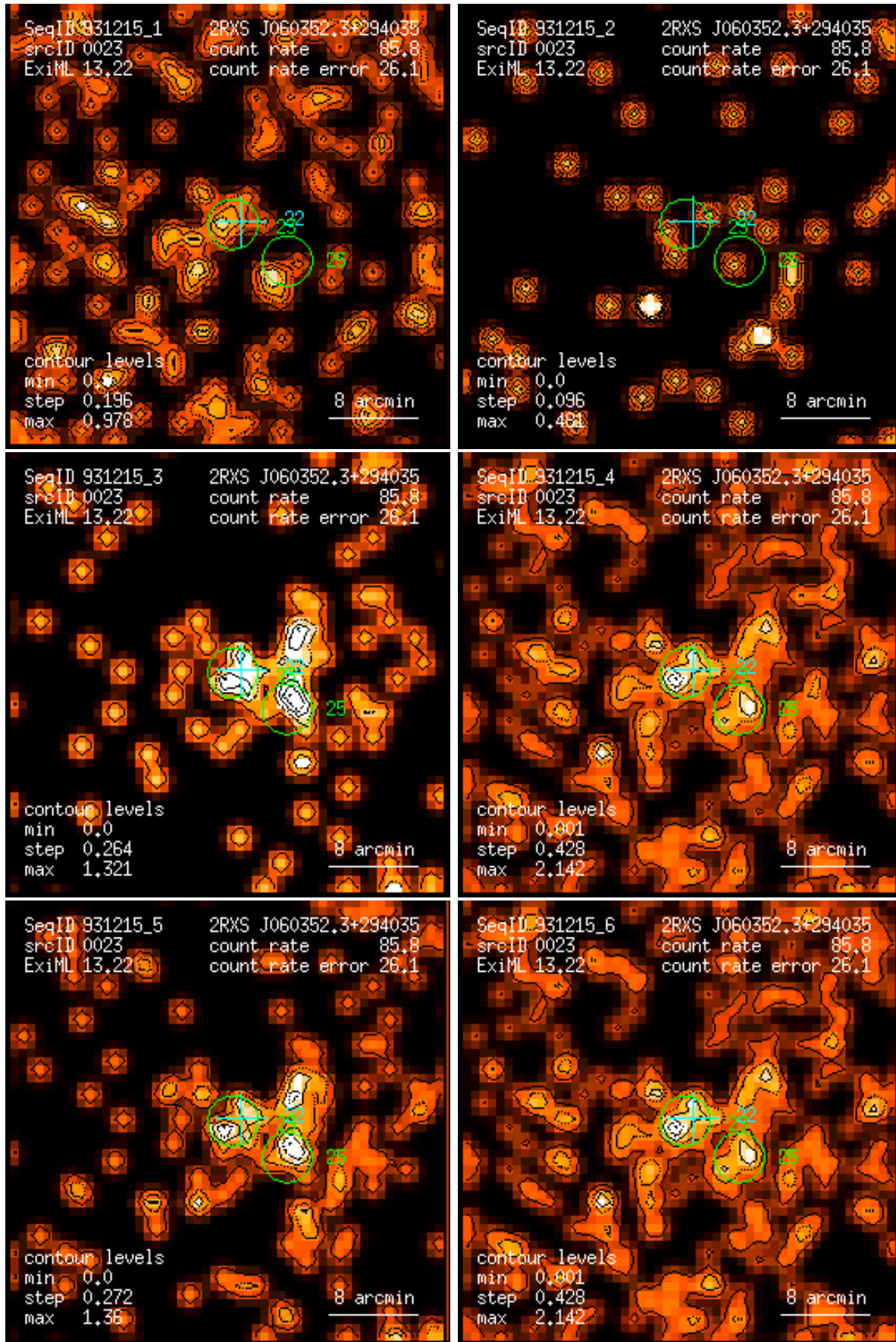
Figure 23: RASS 931215: detection 0023: band rate images, Gaussian filter: (1) PSPC channels 11 – 41, (2) 52 – 90, (3) 91 – 201, (4) 11 – 235, (5) 52 – 201, (6) 11 – 201. Broad band rates in counts/ks. Band rate contour levels in counts/ks/arcmin 2 .
