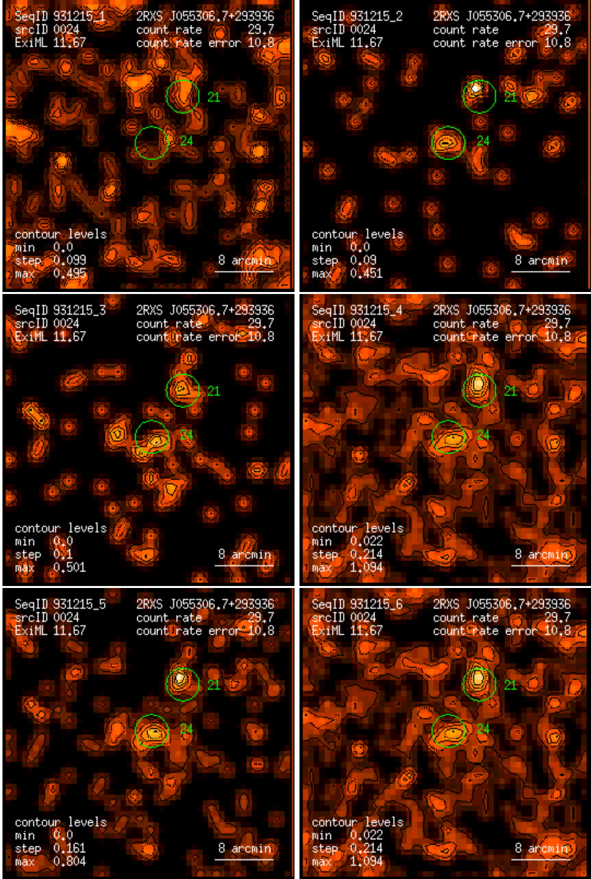
Figure 24: RASS 931215: detection 0024: band rate images, Gaussian filter: (1) PSPC channels 11 – 41, (2) 52 – 90, (3) 91 – 201, (4) 11 – 235, (5) 52 – 201, (6) 11 – 201. Broad band rates in counts/ks. Band rate contour levels in counts/ks/arcmin 2 .
