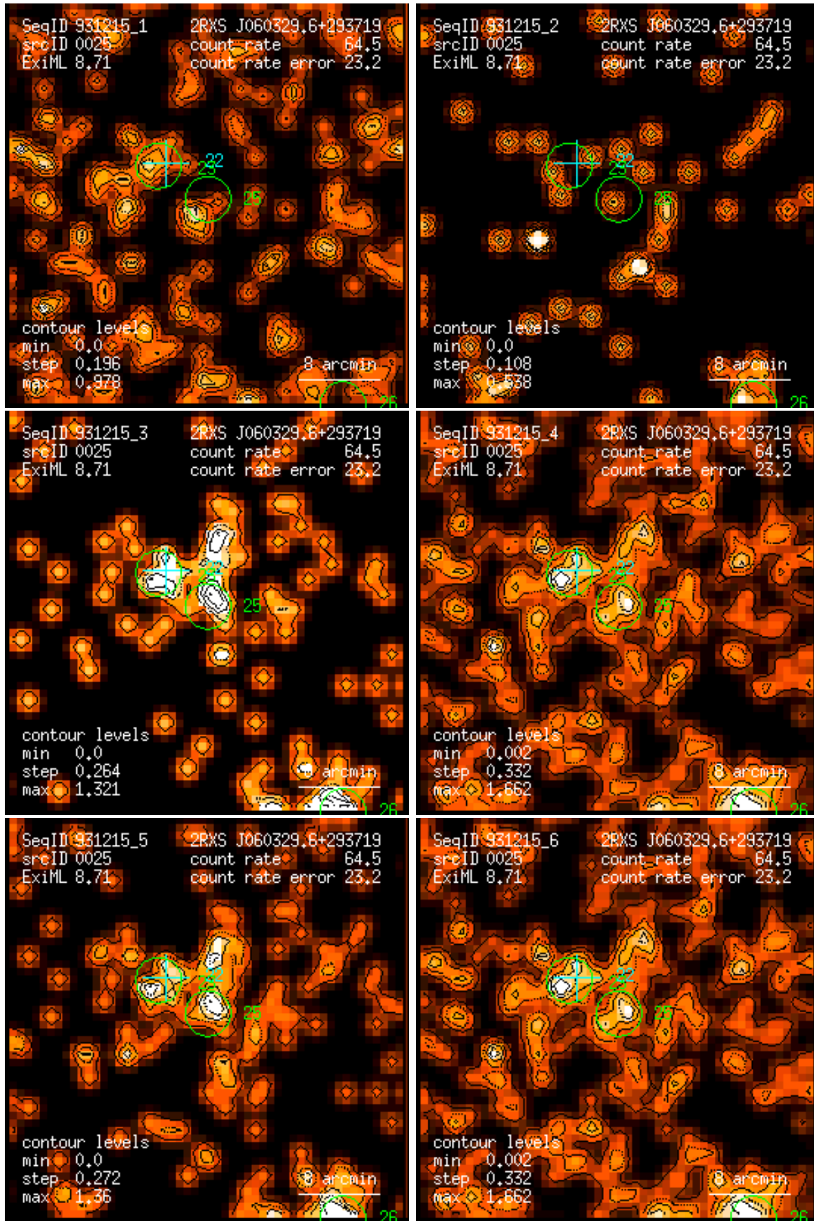
Figure 25: RASS 931215: detection 0025: band rate images, Gaussian filter: (1) PSPC channels 11 – 41, (2) 52 – 90, (3) 91 – 201, (4) 11 – 235, (5) 52 – 201, (6) 11 – 201. Broad band rates in counts/ks. Band rate contour levels in counts/ks/arcmin 2 .
