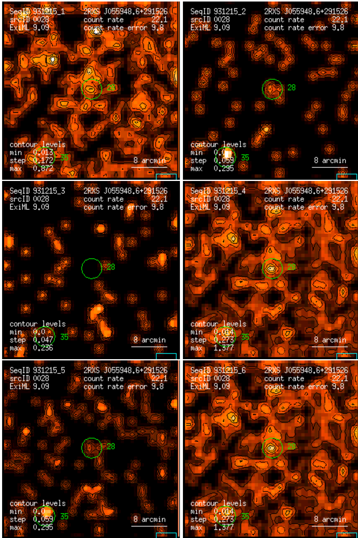
Figure 28: RASS 931215: detection 0028: band rate images, Gaussian filter: (1) PSPC channels 11 – 41, (2) 52 – 90, (3) 91 – 201, (4) 11 – 235, (5) 52 – 201, (6) 11 – 201. Broad band rates in counts/ks. Band rate contour levels in counts/ks/arcmin 2 .
