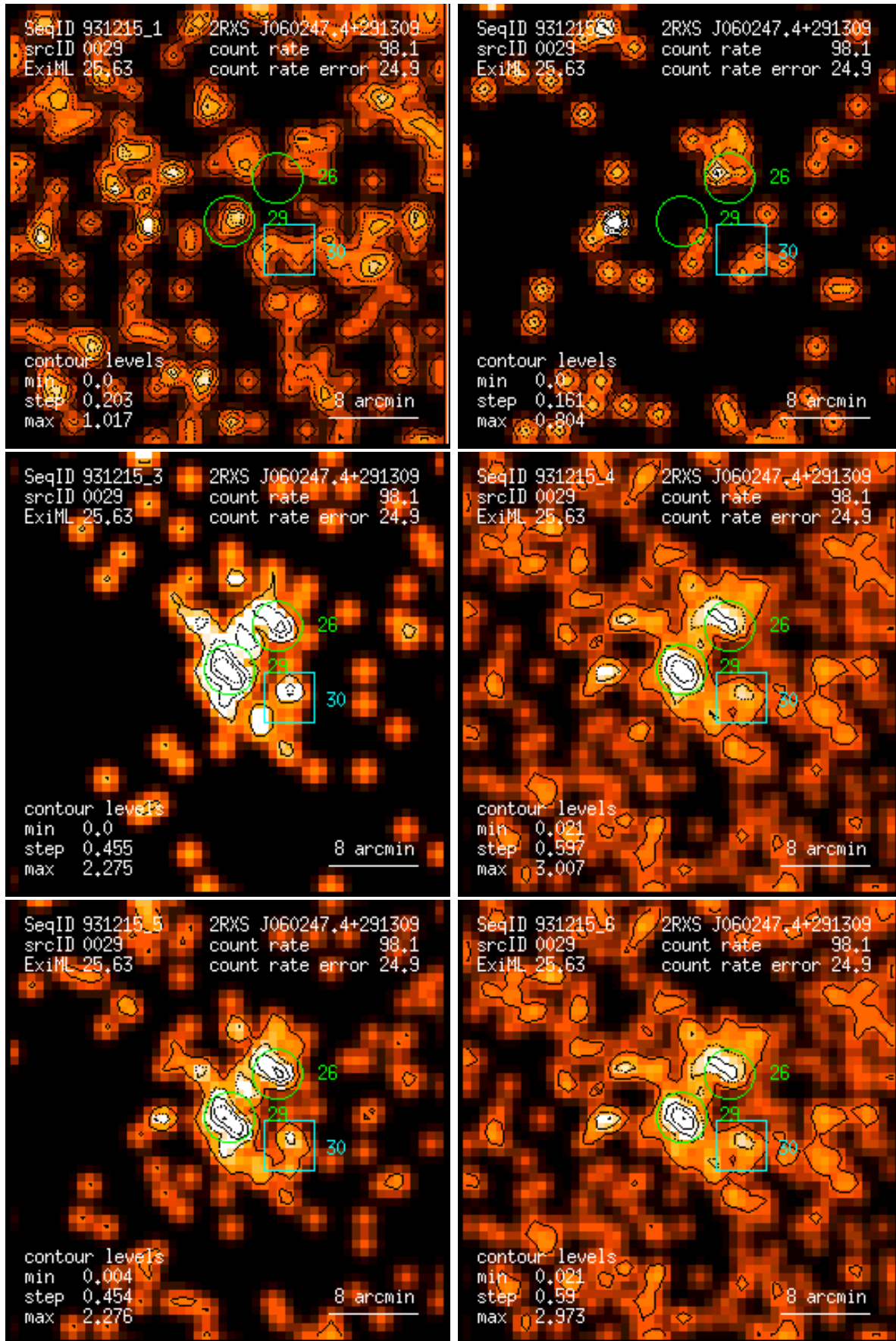
Figure 29: RASS 931215: detection 0029: band rate images, Gaussian filter: (1) PSPC channels 11 – 41, (2) 52 – 90, (3) 91 – 201, (4) 11 – 235, (5) 52 – 201, (6) 11 – 201. Broad band rates in counts/ks. Band rate contour levels in counts/ks/arcmin 2 .
