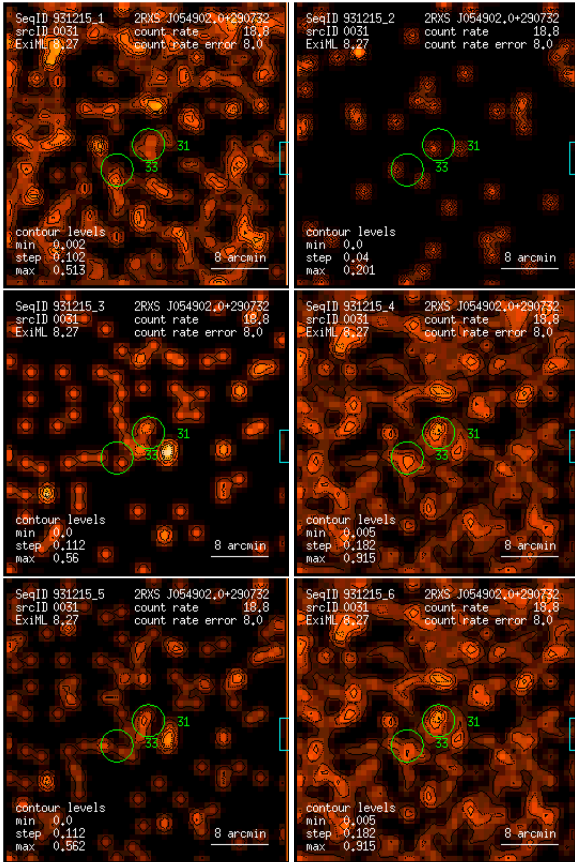
Figure 31: RASS 931215: detection 0031: band rate images, Gaussian filter: (1) PSPC channels 11 – 41, (2) 52 – 90, (3) 91 – 201, (4) 11 – 235, (5) 52 – 201, (6) 11 – 201. Broad band rates in counts/ks. Band rate contour levels in counts/ks/arcmin 2 .
