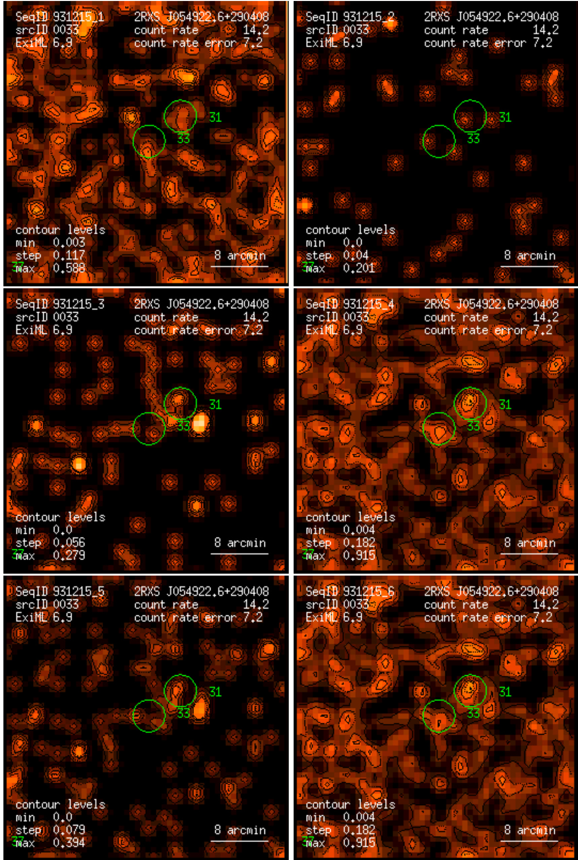
Figure 33: RASS 931215: detection 0033: band rate images, Gaussian filter: (1) PSPC channels 11 – 41, (2) 52 – 90, (3) 91 – 201, (4) 11 – 235, (5) 52 – 201, (6) 11 – 201. Broad band rates in counts/ks. Band rate contour levels in counts/ks/arcmin 2 .
