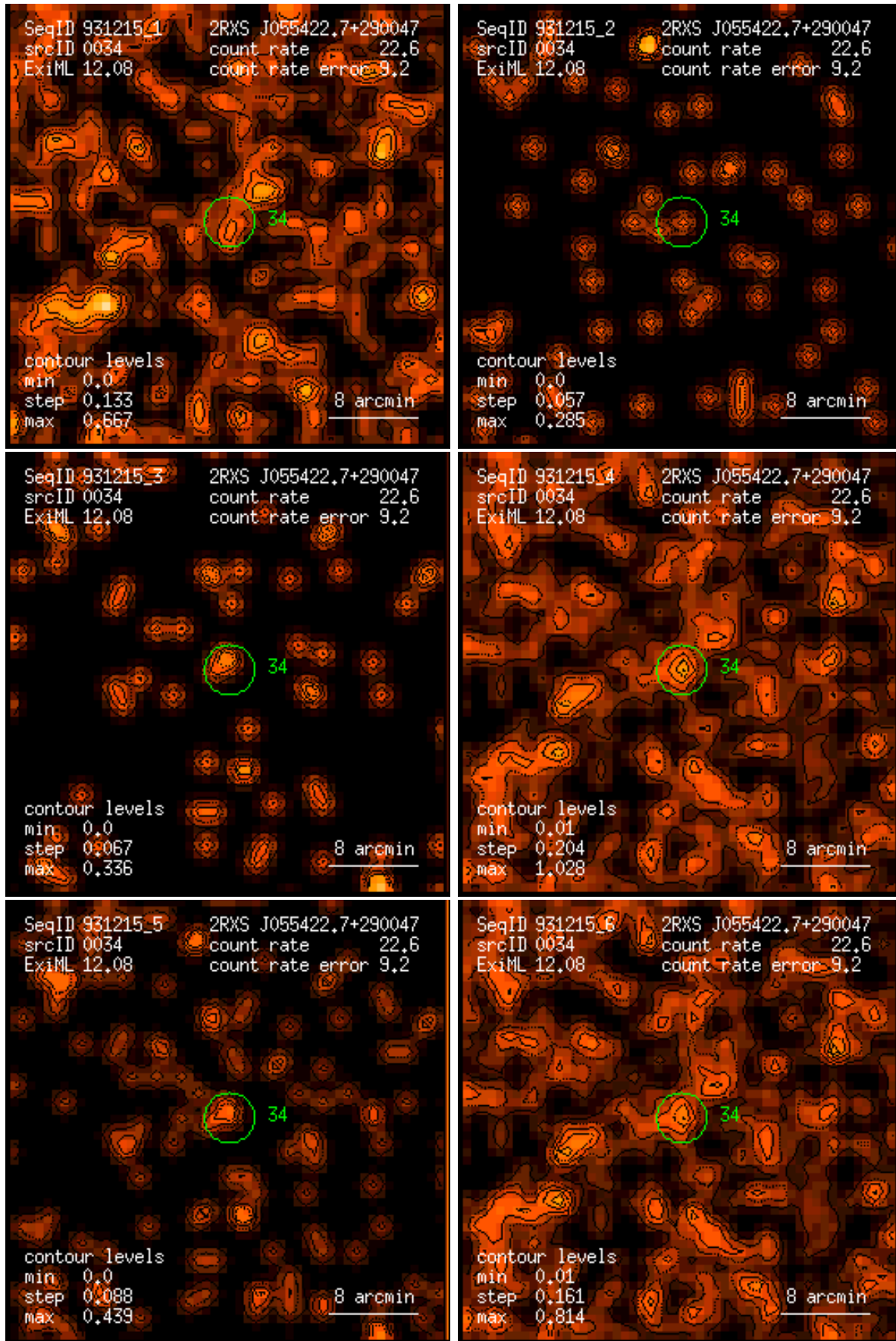
Figure 34: RASS 931215: detection 0034: band rate images, Gaussian filter: (1) PSPC channels 11 – 41, (2) 52 – 90, (3) 91 – 201, (4) 11 – 235, (5) 52 – 201, (6) 11 – 201. Broad band rates in counts/ks. Band rate contour levels in counts/ks/arcmin 2 .
