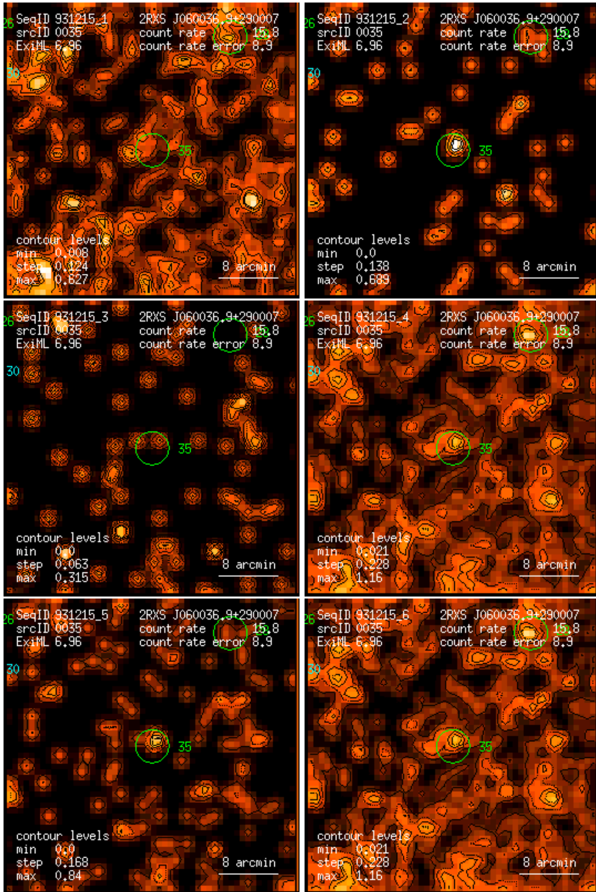
Figure 35: RASS 931215: detection 0035: band rate images, Gaussian filter: (1) PSPC channels 11 – 41, (2) 52 – 90, (3) 91 – 201, (4) 11 – 235, (5) 52 – 201, (6) 11 – 201. Broad band rates in counts/ks. Band rate contour levels in counts/ks/arcmin 2 .
