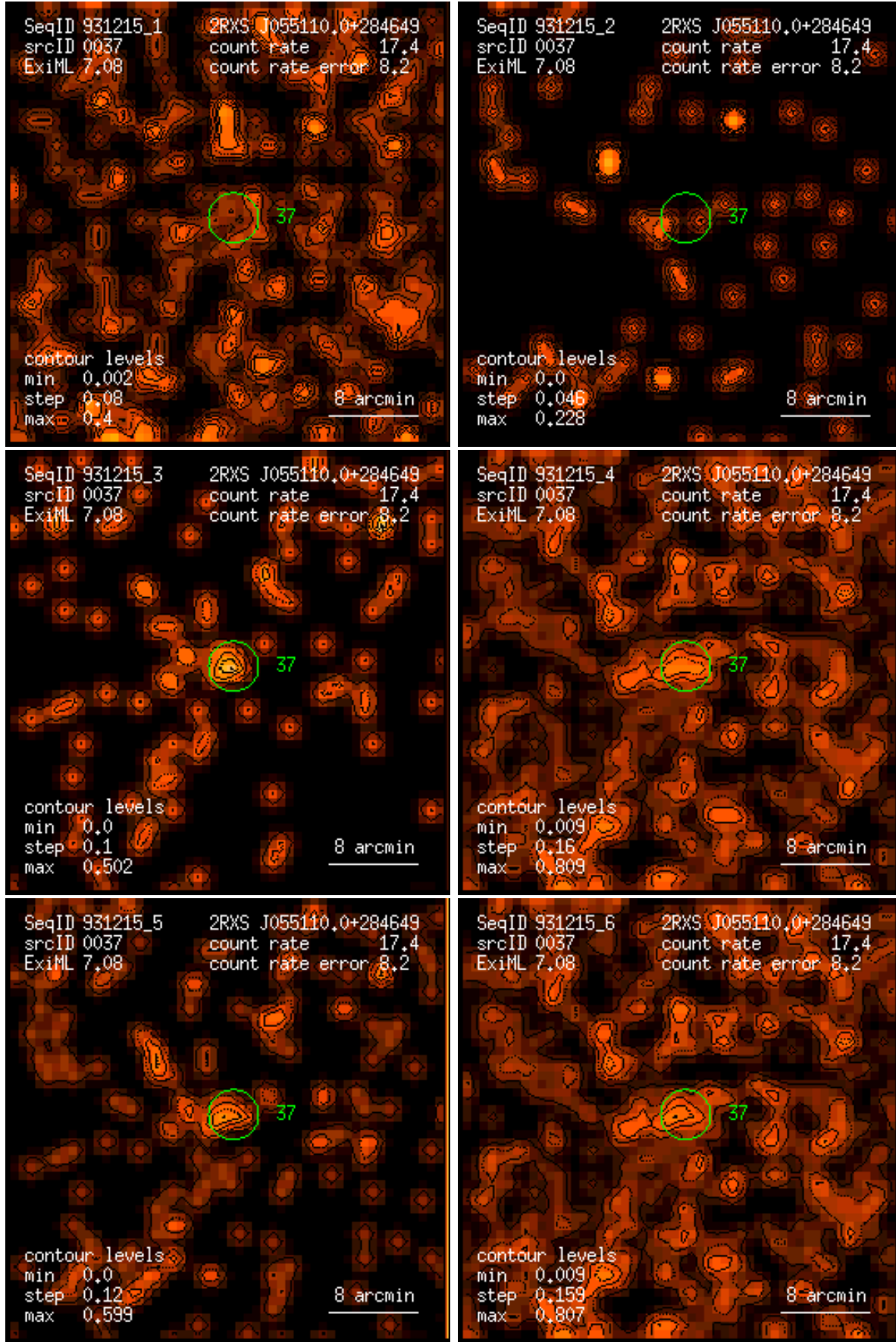
Figure 37: RASS 931215: detection 0037: band rate images, Gaussian filter: (1) PSPC channels 11 – 41, (2) 52 – 90, (3) 91 – 201, (4) 11 – 235, (5) 52 – 201, (6) 11 – 201. Broad band rates in counts/ks. Band rate contour levels in counts/ks/arcmin 2 .
