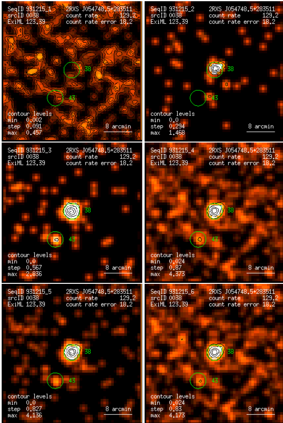
Figure 38: RASS 931215: detection 0038: band rate images, Gaussian filter: (1) PSPC channels 11 – 41, (2) 52 – 90, (3) 91 – 201, (4) 11 – 235, (5) 52 – 201, (6) 11 – 201. Broad band rates in counts/ks. Band rate contour levels in counts/ks/arcmin 2 .
