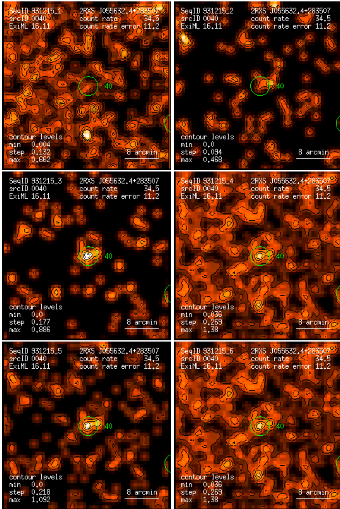
Figure 40: RASS 931215: detection 0040: band rate images, Gaussian filter: (1) PSPC channels 11 – 41, (2) 52 – 90, (3) 91 – 201, (4) 11 – 235, (5) 52 – 201, (6) 11 – 201. Broad band rates in counts/ks. Band rate contour levels in counts/ks/arcmin 2 .
