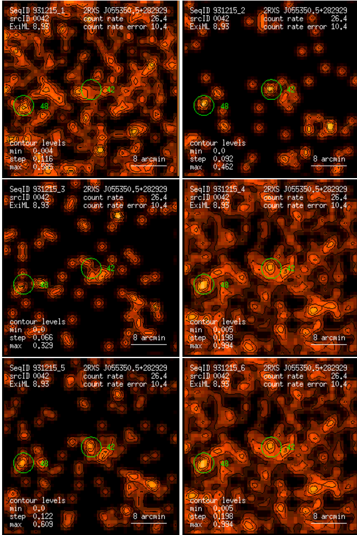
Figure 42: RASS 931215: detection 0042: band rate images, Gaussian filter: (1) PSPC channels 11 – 41, (2) 52 – 90, (3) 91 – 201, (4) 11 – 235, (5) 52 – 201, (6) 11 – 201. Broad band rates in counts/ks. Band rate contour levels in counts/ks/arcmin 2 .
