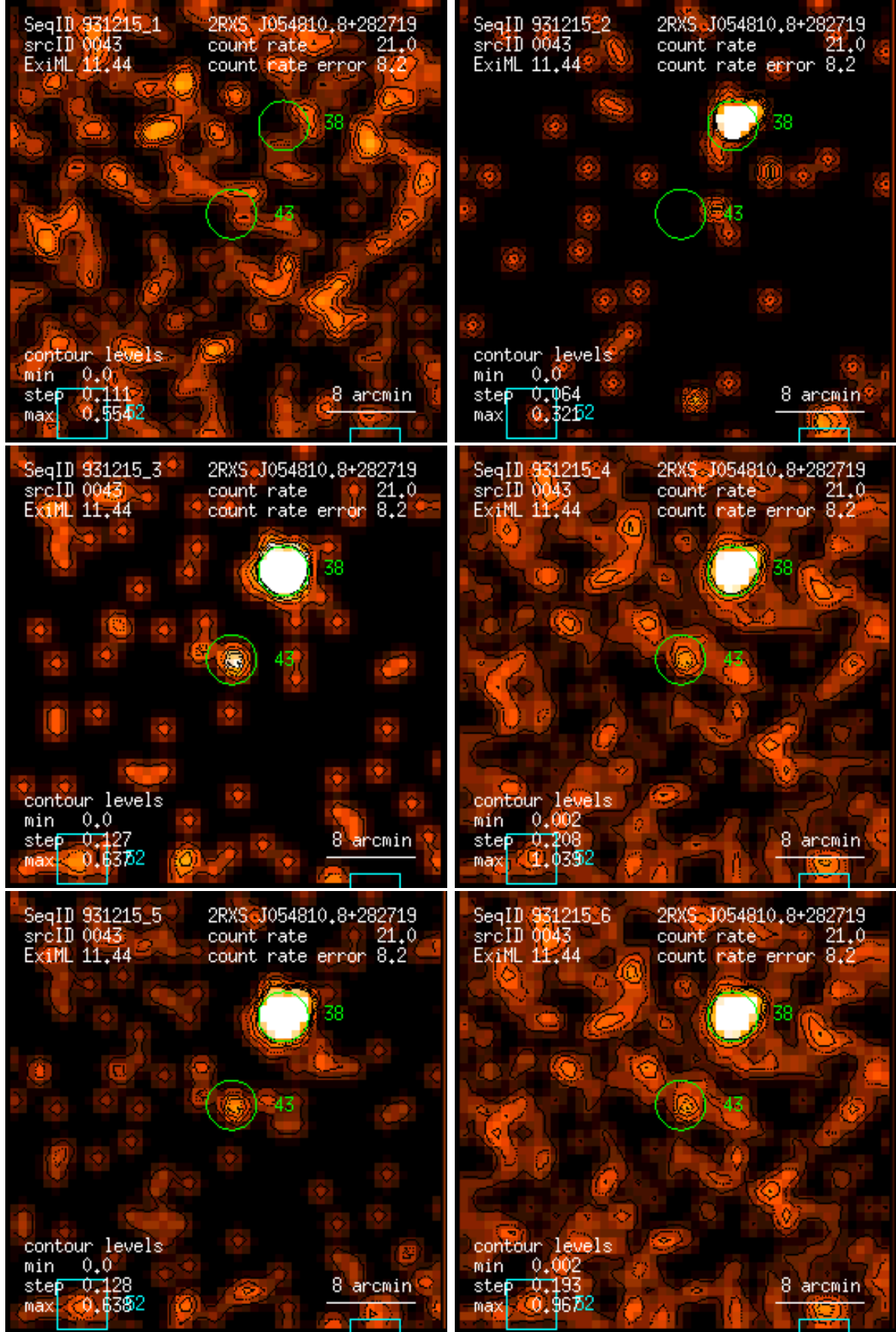
Figure 43: RASS 931215: detection 0043: band rate images, Gaussian filter: (1) PSPC channels 11 – 41, (2) 52 – 90, (3) 91 – 201, (4) 11 – 235, (5) 52 – 201, (6) 11 – 201. Broad band rates in counts/ks. Band rate contour levels in counts/ks/arcmin 2 .
