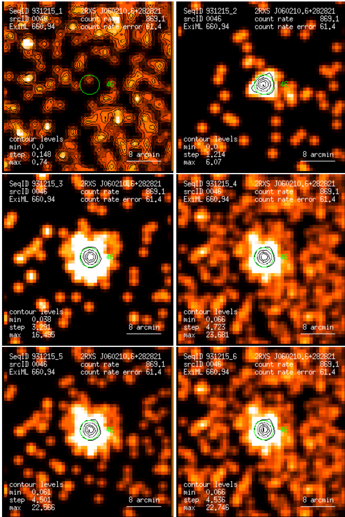
Figure 46: RASS 931215: detection 0046: band rate images, Gaussian filter: (1) PSPC channels 11 – 41, (2) 52 – 90, (3) 91 – 201, (4) 11 – 235, (5) 52 – 201, (6) 11 – 201. Broad band rates in counts/ks. Band rate contour levels in counts/ks/arcmin 2 .
