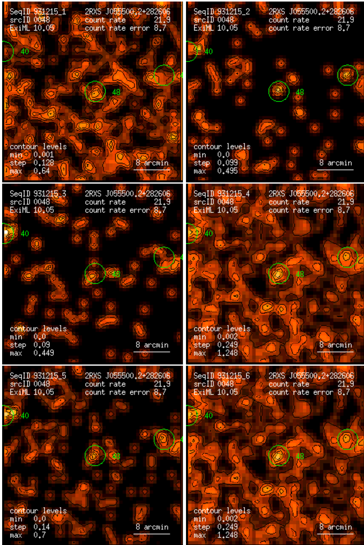
Figure 48: RASS 931215: detection 0048: band rate images, Gaussian filter: (1) PSPC channels 11 – 41, (2) 52 – 90, (3) 91 – 201, (4) 11 – 235, (5) 52 – 201, (6) 11 – 201. Broad band rates in counts/ks. Band rate contour levels in counts/ks/arcmin 2 .
