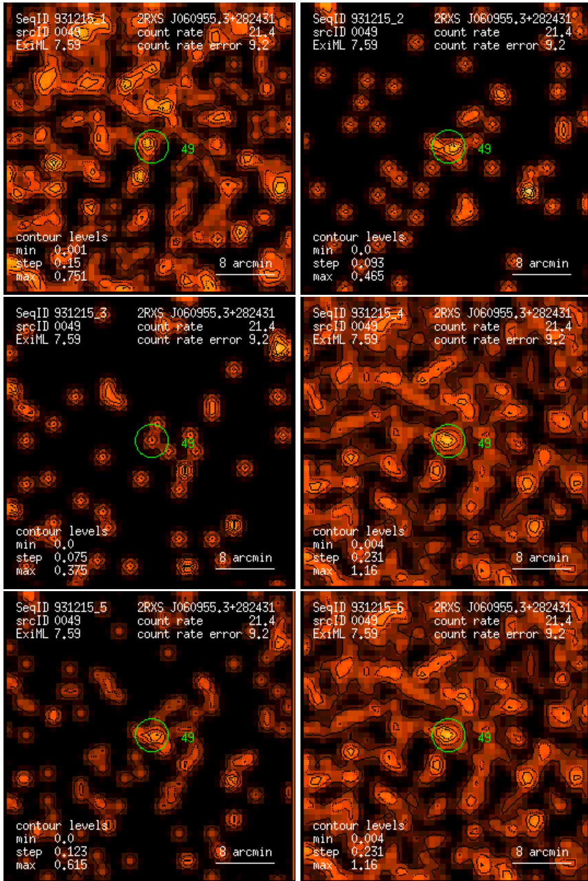
Figure 49: RASS 931215: detection 0049: band rate images, Gaussian filter: (1) PSPC channels 11 – 41, (2) 52 – 90, (3) 91 – 201, (4) 11 – 235, (5) 52 – 201, (6) 11 – 201. Broad band rates in counts/ks. Band rate contour levels in counts/ks/arcmin 2 .
