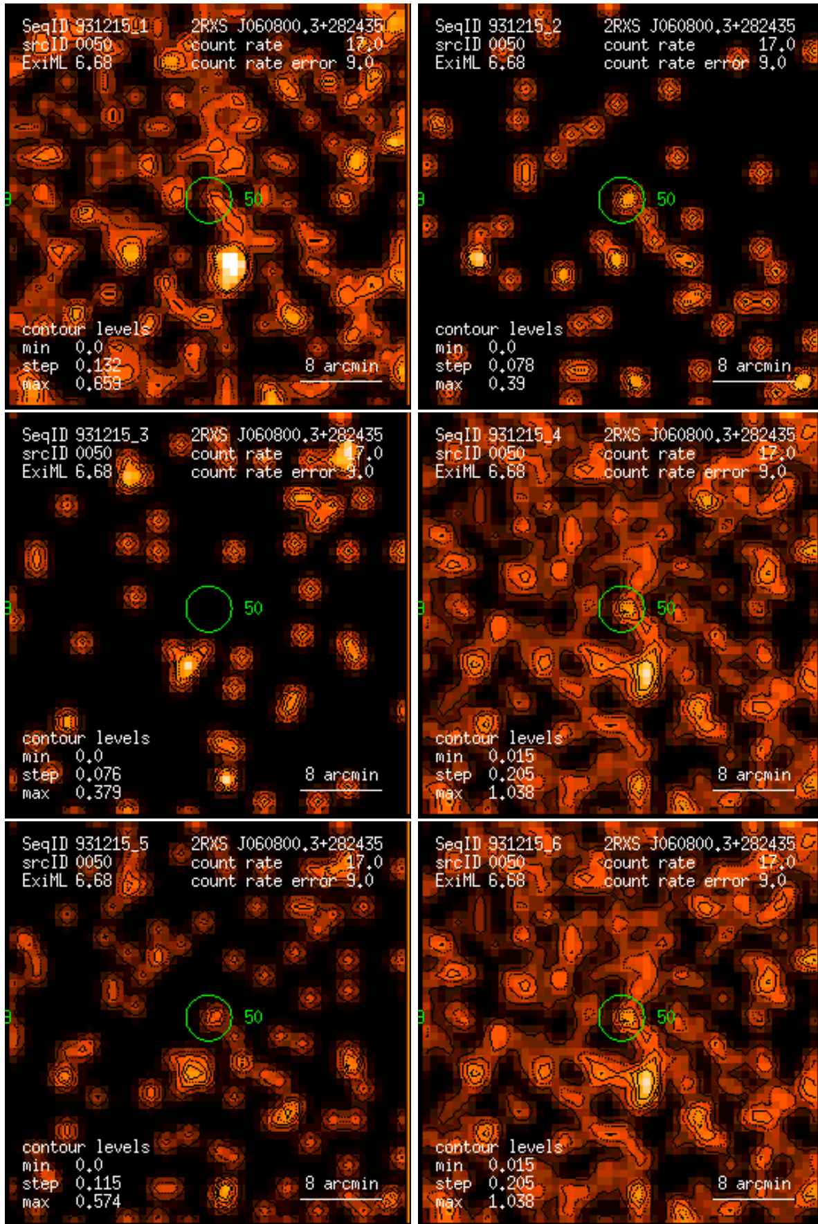
Figure 50: RASS 931215: detection 0050: band rate images, Gaussian filter: (1) PSPC channels 11 – 41, (2) 52 – 90, (3) 91 – 201, (4) 11 – 235, (5) 52 – 201, (6) 11 – 201. Broad band rates in counts/ks. Band rate contour levels in counts/ks/arcmin 2 .
