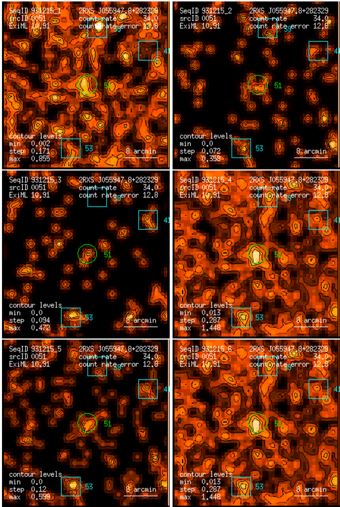
Figure 51: RASS 931215: detection 0051: band rate images, Gaussian filter: (1) PSPC channels 11 – 41, (2) 52 – 90, (3) 91 – 201, (4) 11 – 235, (5) 52 – 201, (6) 11 – 201. Broad band rates in counts/ks. Band rate contour levels in counts/ks/arcmin 2 .
