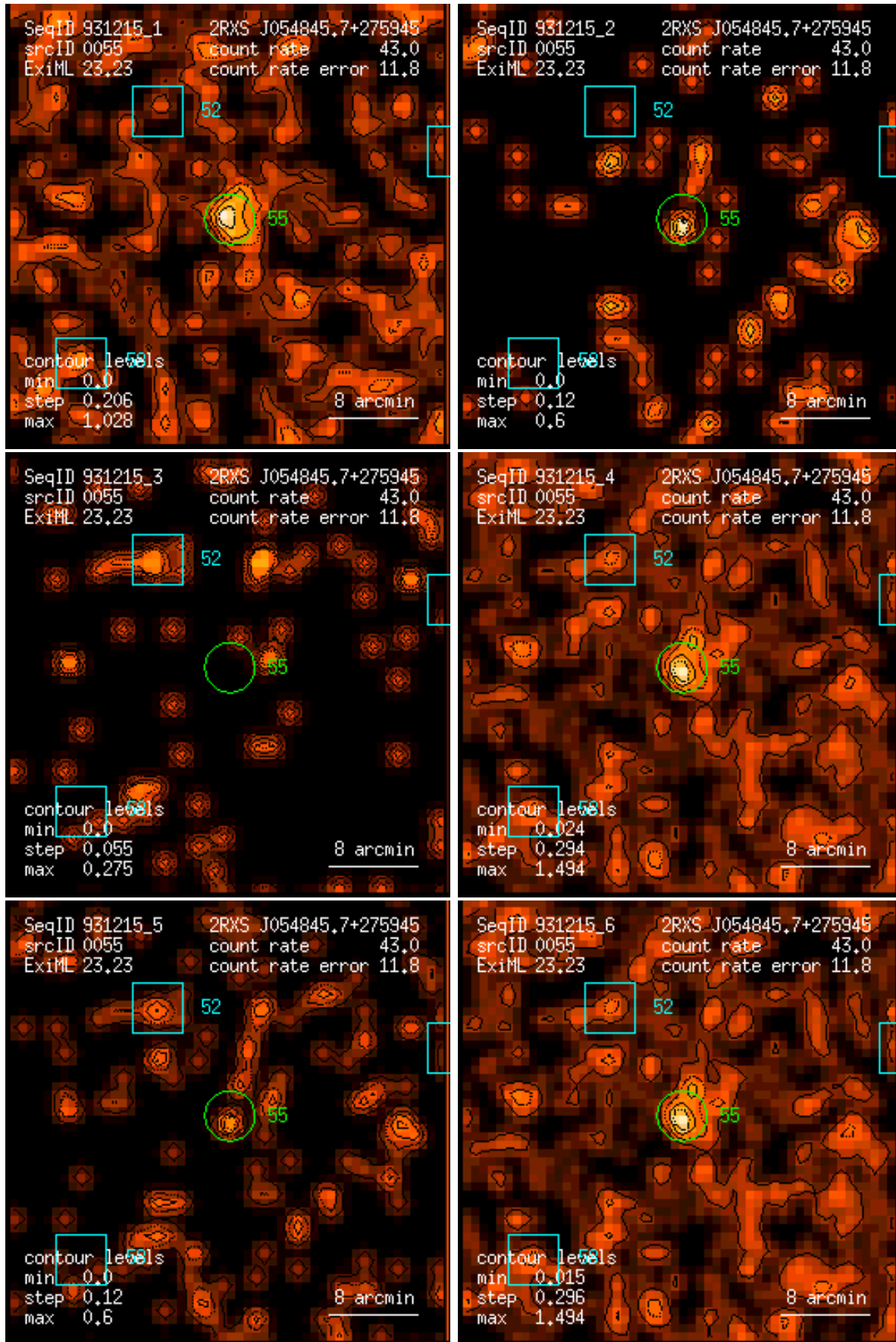
Figure 55: RASS 931215: detection 0055: band rate images, Gaussian filter: (1) PSPC channels 11 – 41, (2) 52 – 90, (3) 91 – 201, (4) 11 – 235, (5) 52 – 201, (6) 11 – 201. Broad band rates in counts/ks. Band rate contour levels in counts/ks/arcmin 2 .
