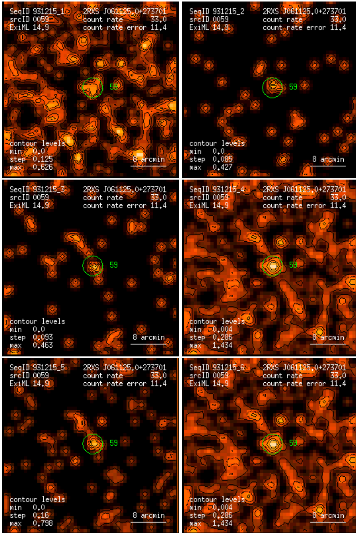
Figure 59: RASS 931215: detection 0059: band rate images, Gaussian filter: (1) PSPC channels 11 – 41, (2) 52 – 90, (3) 91 – 201, (4) 11 – 235, (5) 52 – 201, (6) 11 – 201. Broad band rates in counts/ks. Band rate contour levels in counts/ks/arcmin 2 .
