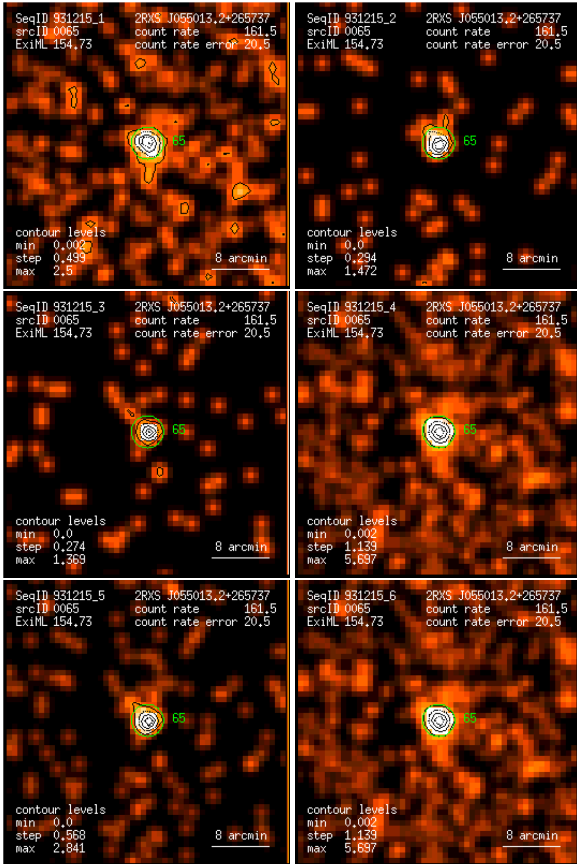
Figure 65: RASS 931215: detection 0065: band rate images, Gaussian filter: (1) PSPC channels 11 – 41, (2) 52 – 90, (3) 91 – 201, (4) 11 – 235, (5) 52 – 201, (6) 11 – 201. Broad band rates in counts/ks. Band rate contour levels in counts/ks/arcmin 2 .
