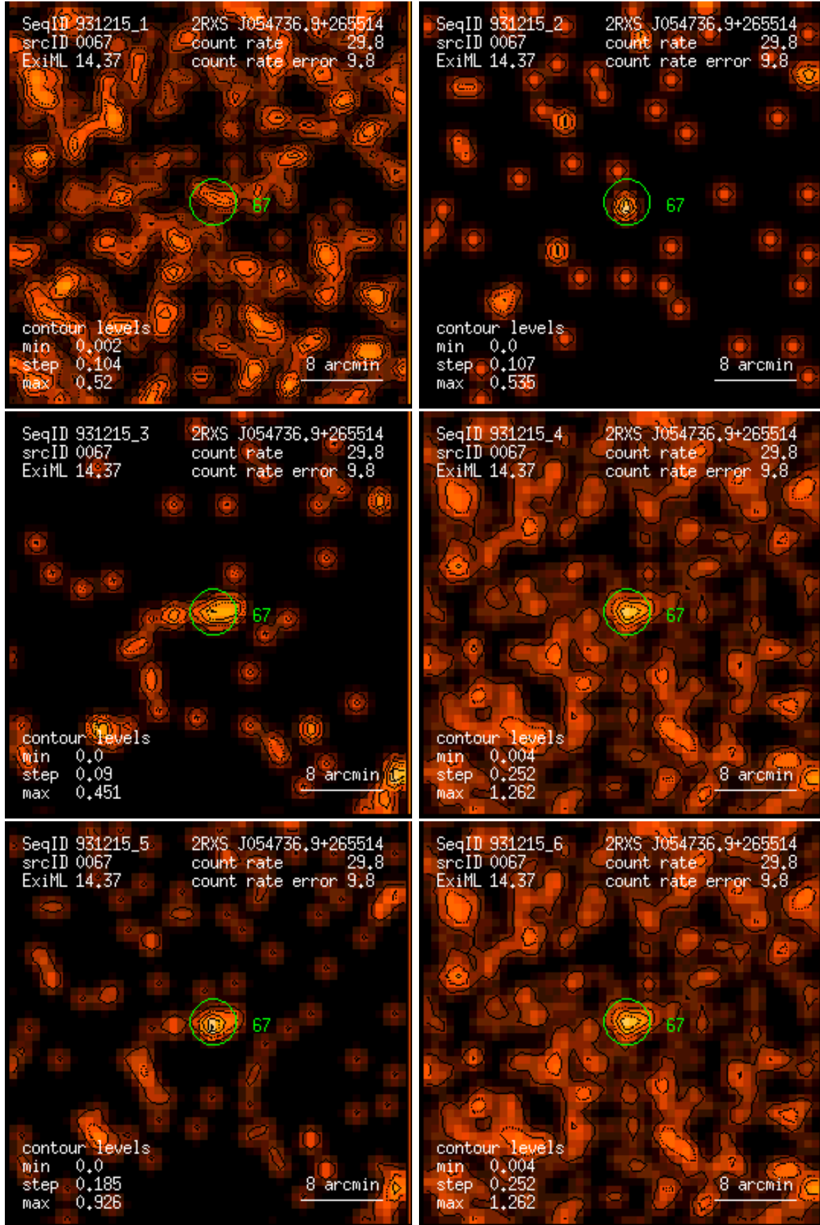
Figure 67: RASS 931215: detection 0067: band rate images, Gaussian filter: (1) PSPC channels 11 – 41, (2) 52 – 90, (3) 91 – 201, (4) 11 – 235, (5) 52 – 201, (6) 11 – 201. Broad band rates in counts/ks. Band rate contour levels in counts/ks/arcmin 2 .
