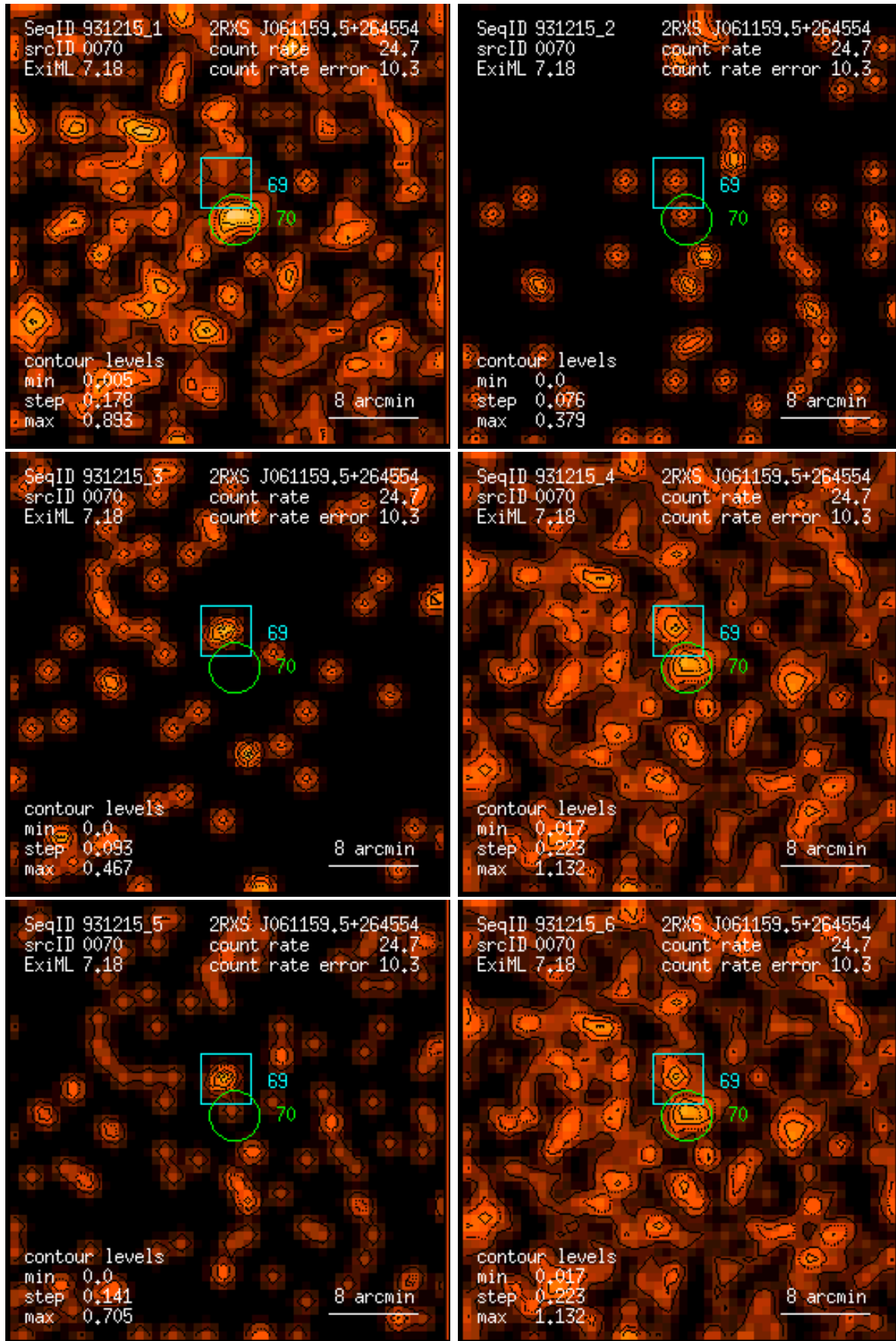
Figure 70: RASS 931215: detection 0070: band rate images, Gaussian filter: (1) PSPC channels 11 – 41, (2) 52 – 90, (3) 91 – 201, (4) 11 – 235, (5) 52 – 201, (6) 11 – 201. Broad band rates in counts/ks. Band rate contour levels in counts/ks/arcmin 2 .
