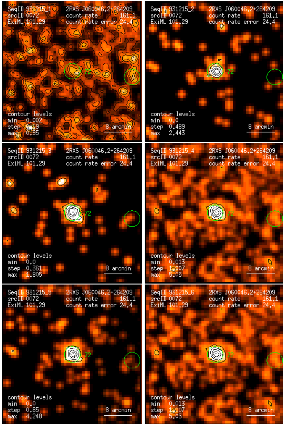
Figure 72: RASS 931215: detection 0072: band rate images, Gaussian filter: (1) PSPC channels 11 – 41, (2) 52 – 90, (3) 91 – 201, (4) 11 – 235, (5) 52 – 201, (6) 11 – 201. Broad band rates in counts/ks. Band rate contour levels in counts/ks/arcmin 2 .
