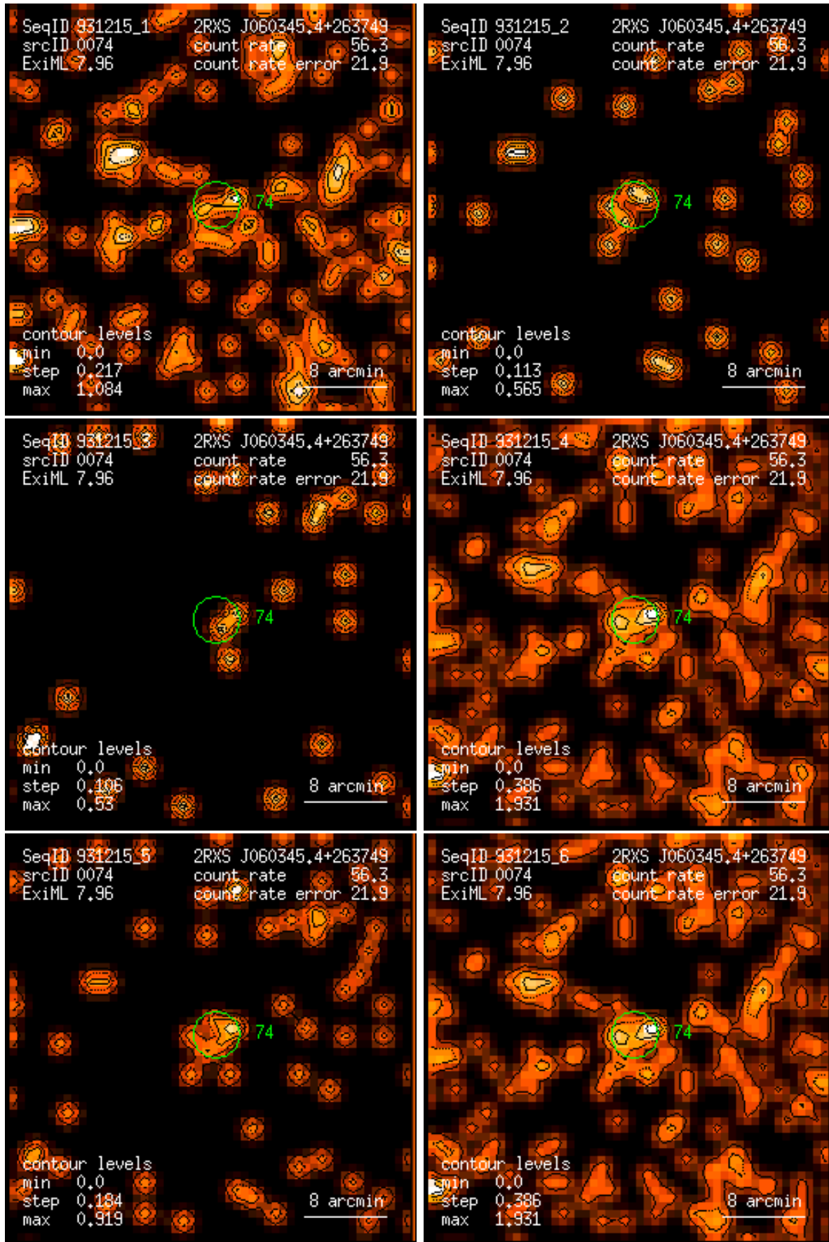
Figure 74: RASS 931215: detection 0074: band rate images, Gaussian filter: (1) PSPC channels 11 – 41, (2) 52 – 90, (3) 91 – 201, (4) 11 – 235, (5) 52 – 201, (6) 11 – 201. Broad band rates in counts/ks. Band rate contour levels in counts/ks/arcmin 2 .
