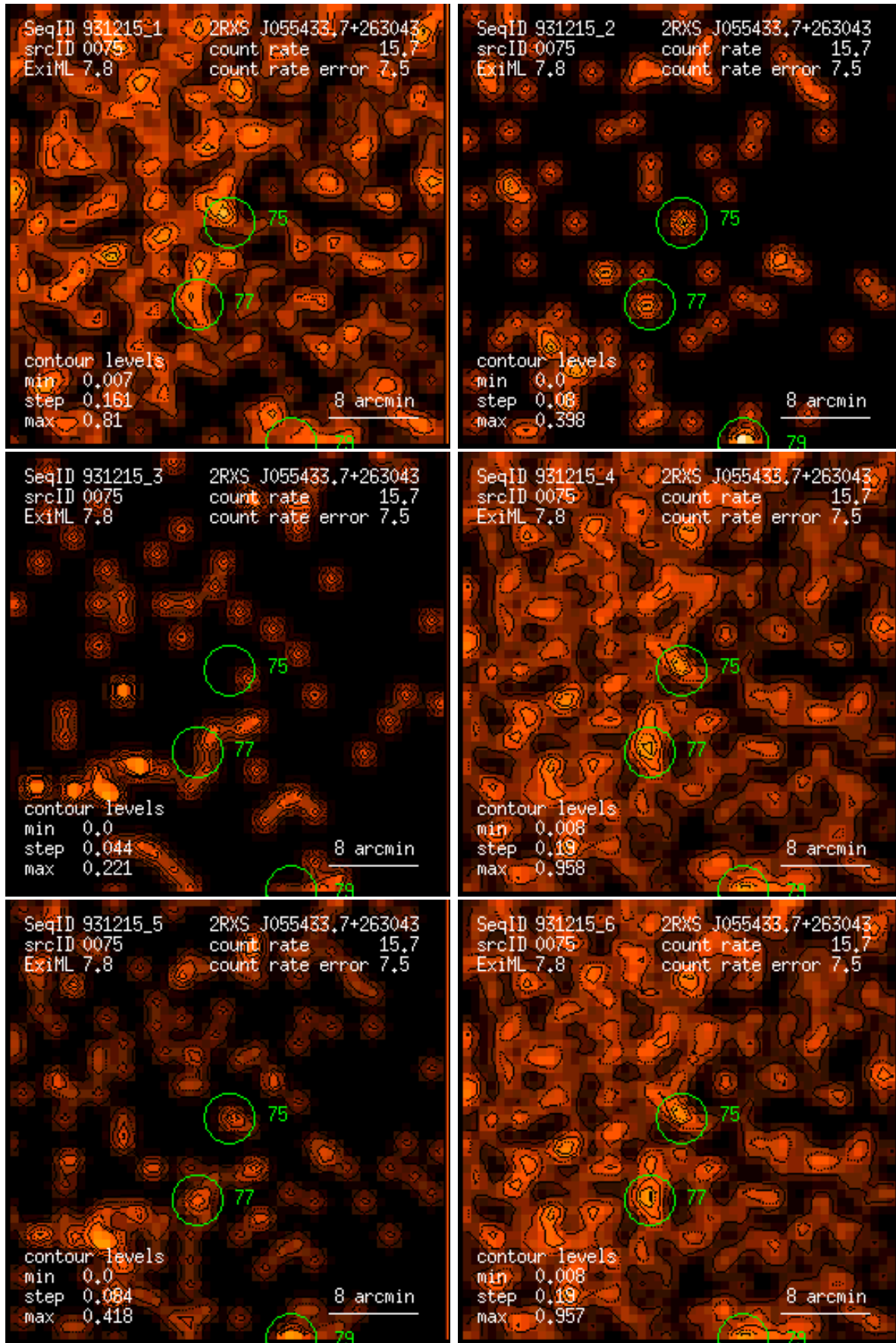
Figure 75: RASS 931215: detection 0075: band rate images, Gaussian filter: (1) PSPC channels 11 – 41, (2) 52 – 90, (3) 91 – 201, (4) 11 – 235, (5) 52 – 201, (6) 11 – 201. Broad band rates in counts/ks. Band rate contour levels in counts/ks/arcmin 2 .
