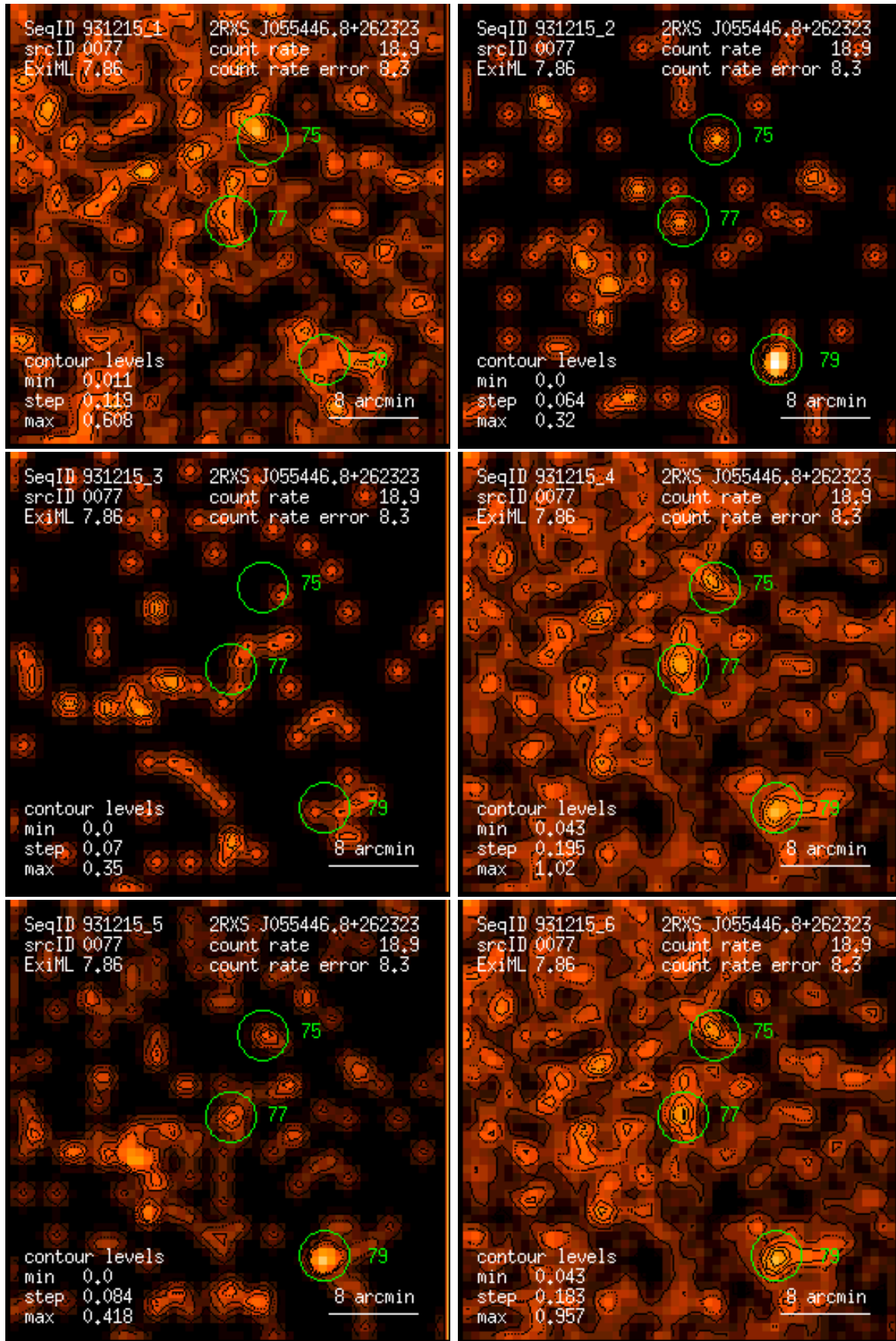
Figure 77: RASS 931215: detection 0077: band rate images, Gaussian filter: (1) PSPC channels 11 – 41, (2) 52 – 90, (3) 91 – 201, (4) 11 – 235, (5) 52 – 201, (6) 11 – 201. Broad band rates in counts/ks. Band rate contour levels in counts/ks/arcmin 2 .
